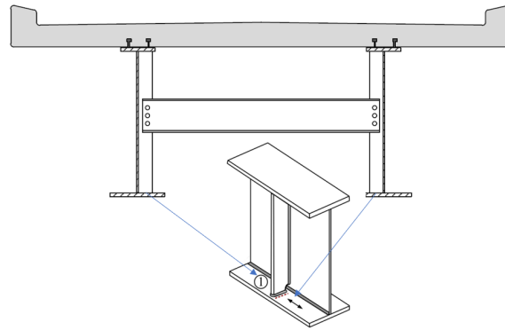
Figure 20. Cross-section of the road bridge girders, the concrete deck, and the transverse detail under study. Figure adapted from [17].
