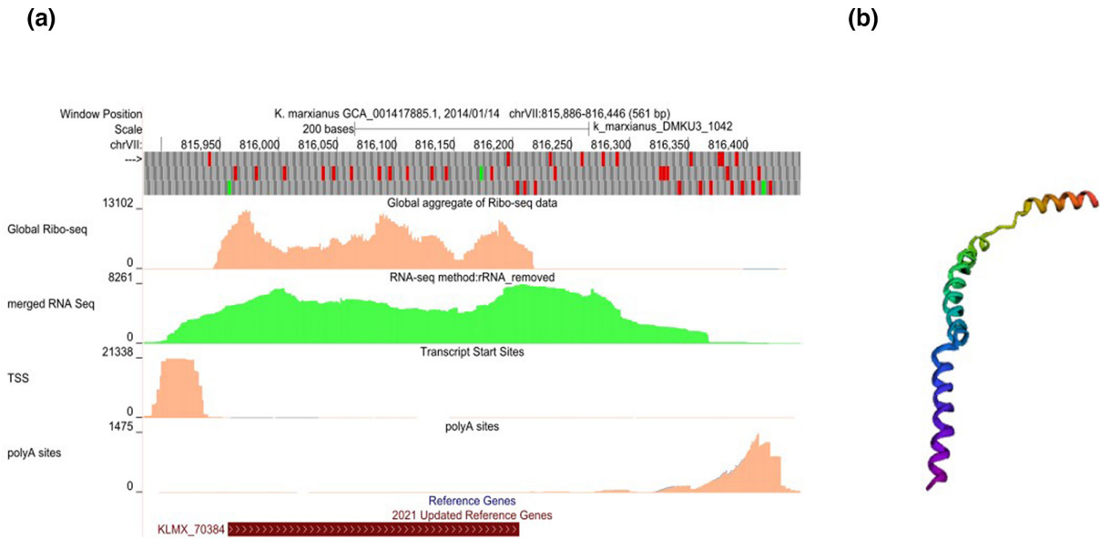
Fig. 4. Transcription, translation and structure of KLMX_70384. (a) GWIPS-viz view of KLMX_70384 showing, from top to bottom: global ribo-seq reads (scale: 0–13 102); merged RNA-seq reads (scale: 0–8261); transcription start sites (TSS, scale: 0–21338); polyA sites (scale: 0–1475). The CDS position is indicated by the red bar on the bottom track. (b) Ab initio prediction of the tertiary structure of the KLMX_70384 protein with Robetta. Structure prediction is predominantly \alpha -helical. Colour in the figure is from blue (N terminus) to red (C terminus).
