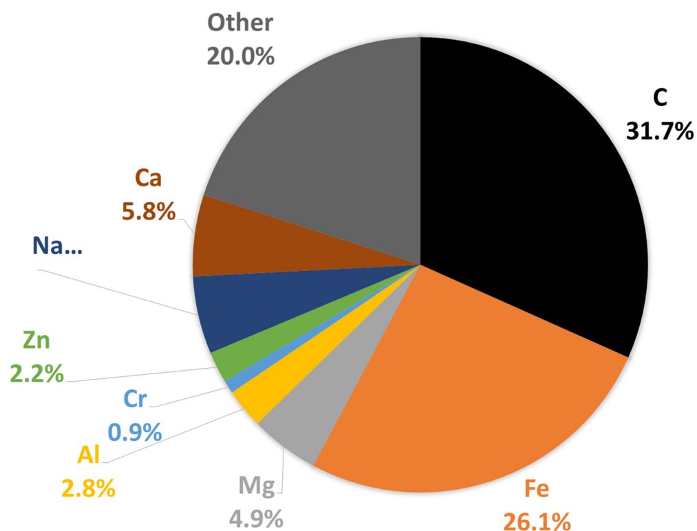
Figure 4. Typical elemental composition of diesel particles using laser-induced breakdown spectroscopy (LIBS). C: carbon, Fe: iron, Mg: magnesium, Al: aluminium, Zn: zinc, Na: sodium, and Ca: calcium (from Viskup et al. [78]).
