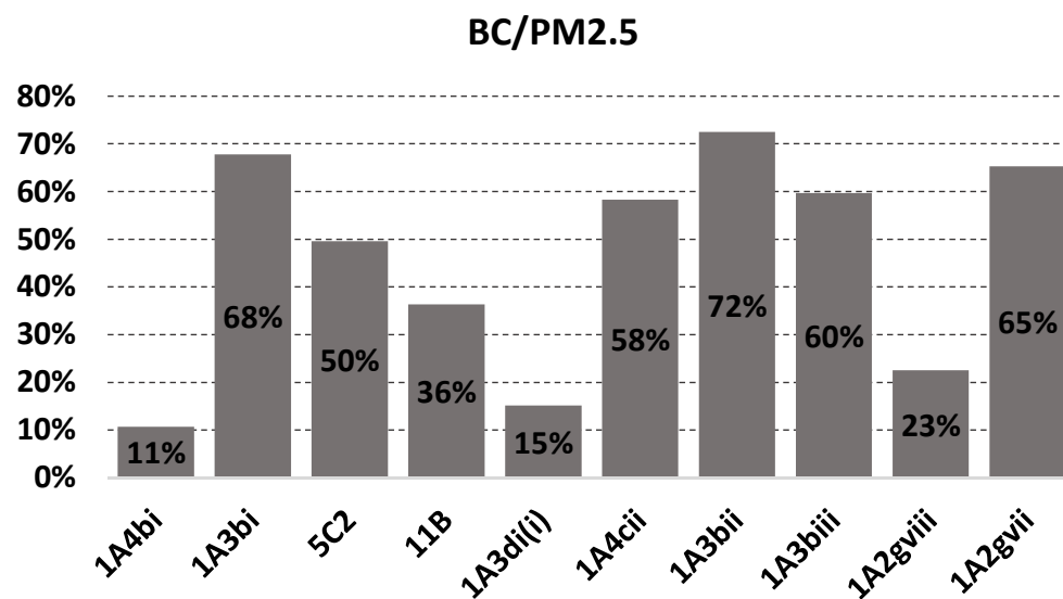
Figure 3. Ratio \text{BC}/\text{PM}_{2.5} for EU28 official emissions in 2018 computed from the EMEP database [53] for the main emitting NFR sectors (refer to Table 3).
