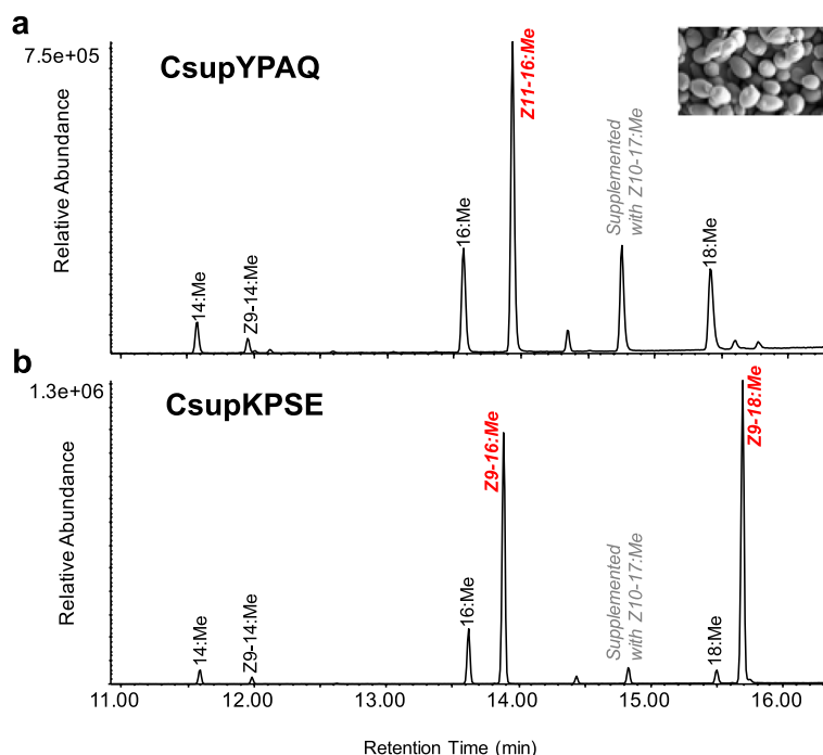
Fig. 2 Heterologous expression of fatty acyl desaturase candidates from Chilo suppressalis in \Delta ole1/elo1 Saccharomyces cerevisiae . GC/MS analysis of fatty acid methyl ester profiles of yeast expressing the CsupYPAQ or CsupKPSE . The compounds produced from the introduced desaturases are labeled in red italics. Methyl (Z)-10-heptadecenoate (Z10-17:Me) was supplemented as nutrition to all the incubations. Displayed chromatograms are representative examples of at least six replicates
