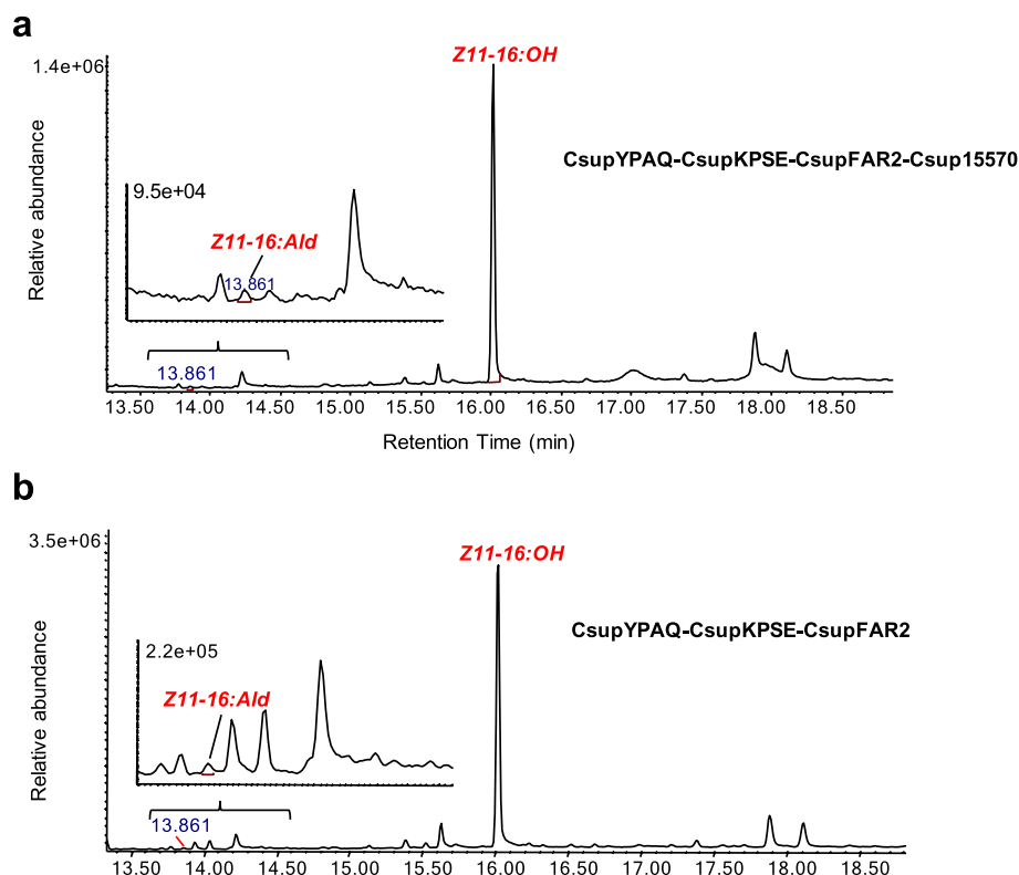
Fig. 7 Heterologous expression of fatty alcohol oxidase candidate Csup15570 with desaturase genes CsupYPAQ and CsupKPSE and reductase gene CsupFAR2 from Chilo suppressalis in Nicotiana benthamiana . GC/MS analysis of Z11-16 fatty alcohol and aldehyde from plant leaves expressing a CsupYPAQ-CsupKPSE-CsupFAR2-Csup15570 and b CsupYPAQ-CsupKPSE-CsupFAR2 . Fatty alcohol and aldehyde are shown in red. Displayed chromatograms are representative examples of at least six replicates
