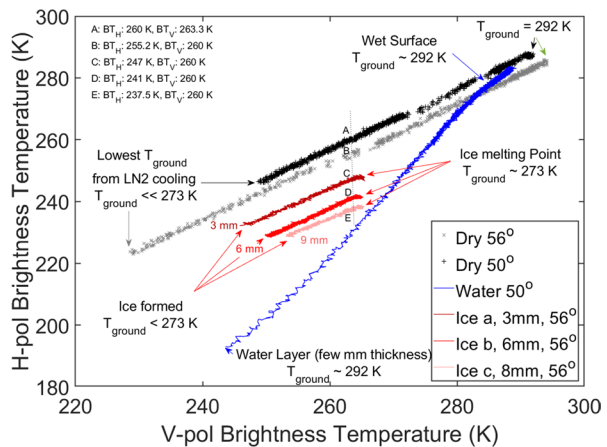
Fig. 8 Measured H-pol–V-pol brightness temperatures for dry asphalt, liquid water, and ice with observation angles of 50° and 56°
