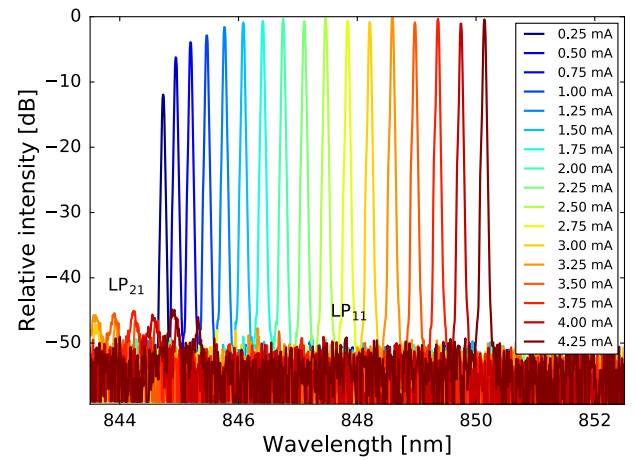
Fig. 9. Output spectrum of a waveguide-coupled VCSIL. The current-induced self-heating results in a wavelength shift close to 5 nm. Mode-selective feedback helps to suppress the first higher-order LP 11 mode with respect to the LP 21 mode.
