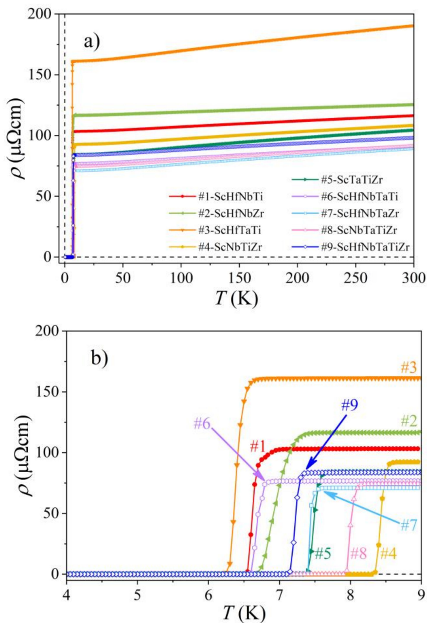
Figure 4. (a) Electrical resistivity of the Sc-Hf-Nb-Ta-Ti-Zr alloys in the temperature range 0.35–300 K. (b) Resistivities on an expanded temperature scale below 9 K.
