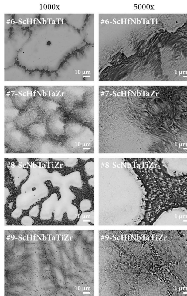
Figure 2. SEM BSE images of the Sc-Hf-Nb-Ta-Ti-Zr alloys #1–#9 at two magnifications, 1000× ( left column) and 5000× ( right column).
