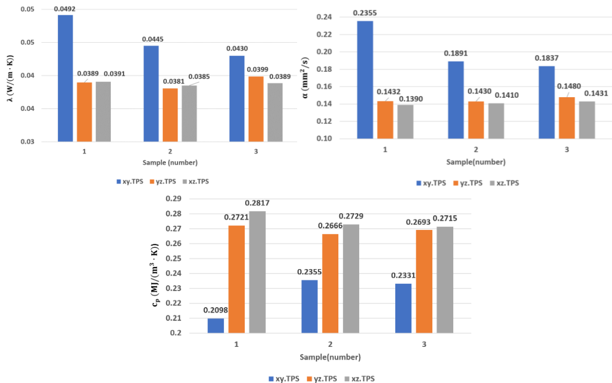
Figure 2. The results from the conducted standard TPS-measurements (average of 40 measurements) for sample sets 1-3 and for measurements of \lambda ( W/(m \cdot K) ) and \alpha ( mm^2/s ). The presented values for c_p ( MJ/(m^3 \cdot K) ) were calculated by the TPS-instrument. The labels describe the position of the TPS sensor for the considered measurement. “xy.TPS”: Measured thermal properties by TPS, in the plane of the sensor, at which the sensor was positioned on plane x-y, see figure 1 (right).
