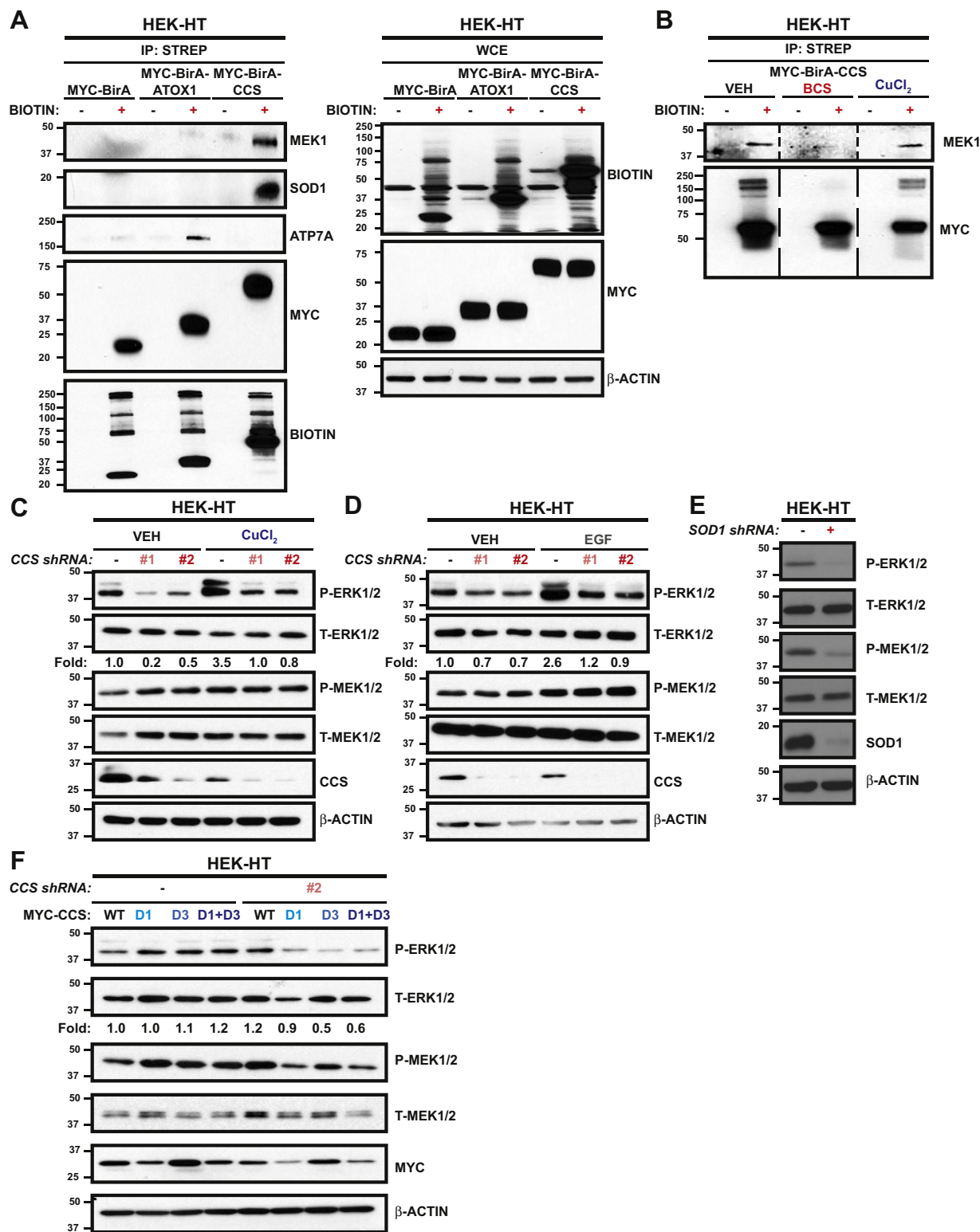
Figure 2. CCS is the necessary Cu chaperone for MEK1. A , immunoblot detection of biotinylated MEK1, ATP7A, SOD1, MYC-BirA, MYC-BirA-ATOX1, or MYC-BirA-CCS from strepavadin pull-downs and whole cell extracts from HEK-HT cells stably expressing MYC-BirA, MYC-BirA-ATOX1, or MYC-BirA-CCS treated with media with (+) or without (-) biotin for 48 h. n = 2 biologically independent experiments. B , immunoblot detection of biotinylated MEK1 or MYC-BirA-CCS from strepavadin pull-downs from HEK-HT cells stably expressing MYC-BirA-CCS treated with media with (+) or without (-) biotin for 48 h in the presence of vehicle, 500 μM bathocuproinedisulfonic acid (BCS), or 1 μM CuCl 2 . n = 2 biologically independent experiments. C and D , immunoblot detection of phosphorylated (P)-ERK1/2, total (T)-ERK1/2, P-MEK1/2, T-MEK1/2, CCS, or β-ACTIN from HEK-HT cells stably expressing doxycycline inducible shRNA against control (-) or CCS (#1 or #2) treated with doxycycline for 24 h followed by (B), vehicle (VEH) or 1 μM CuCl 2 for 20 min or (C), VEH or 0.1 ng/ml EGF for 15 min. Quantification: Fold change P-ERK1/2/T-ERK1/2 normalized to control, VEH. n = 3 biologically independent experiments. E , immunoblot detection of P-ERK1/2, T-ERK1/2, P-MEK1/2, T-MEK1/2, SOD1, or β-ACTIN from HEK-HT cells stably expressing doxycycline inducible shRNA against control (-) or SOD1 (+) treated with doxycycline for 48 h n = 2 biologically independent experiments. F , immunoblot detection of P-ERK1/2, T-ERK1/2, P-MEK1/2, T-MEK1/2, MYC, or β-ACTIN from HEK-HT cells stably expressing doxycycline inducible shRNA against control (-) or CCS (#1 or #2) treated with doxycycline for 24 h followed by (B), vehicle (VEH) or 1 μM CuCl 2 for 20 min or (C), VEH or 0.1 ng/ml EGF for 15 min. Quantification: Fold change P-ERK1/2/T-ERK1/2 normalized to control, VEH. n = 3 biologically independent experiments.
