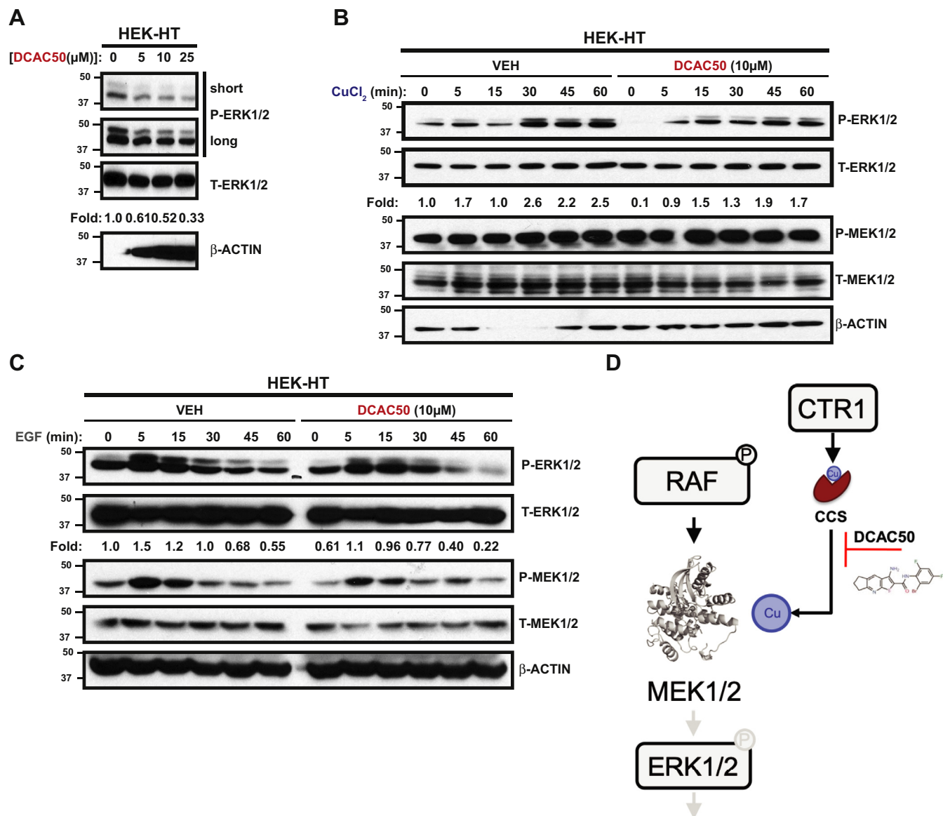
Figure 3. Treatment with small molecular inhibitor of CCS blunts MAPK pathway activation at the level of MEK1/2. A , immunoblot detection of phosphorylated (P)-ERK1/2, total (T)-ERK1/2, or β-ACTIN from HEK-HT cells treated with vehicle (0) or increasing concentrations of DCAC50 for 24 h. Quantification: Fold change P-ERK1/2/T-ERK1/2 normalized to control, VEH. n = 3 biologically independent experiments. B and C , immunoblot detection of P-ERK1/2, T-ERK1/2, P-MEK1/2, T-MEK1/2, or β-ACTIN from HEK-HT cells treated with vehicle (–) or 10 μM DCAC50 for 24 h followed stimulation with ( B ), 1 μM CuCl 2 or ( C ), 0.1 ng/ml EGF for indicated time. Quantification: Fold change P-ERK1/2/T-ERK1/2 normalized to control, VEH. n = 3 biologically independent experiments. D , model of CCS-mediated Cu activation of MEK1/2. CCS, Cu chaperone for superoxide dismutase; Cu, copper; EGF, epidermal growth factor; MAPK, mitogen-associated protein kinase; VEH, vehicle.
