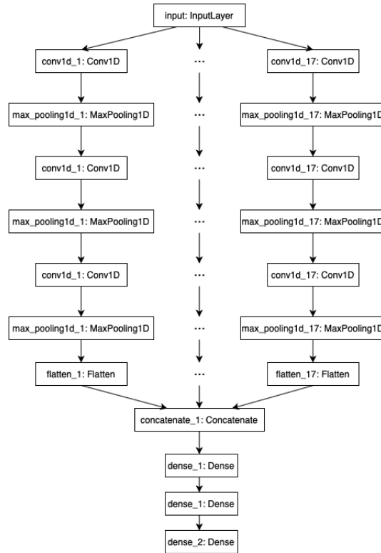
Figure 11: Structure of the CNN model.
