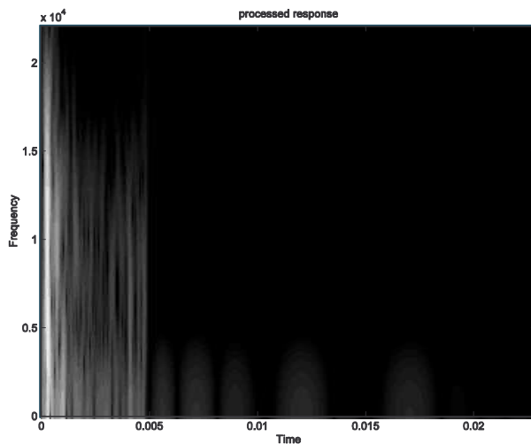
Figure 28. H-FDTW impulse response spectrogram
