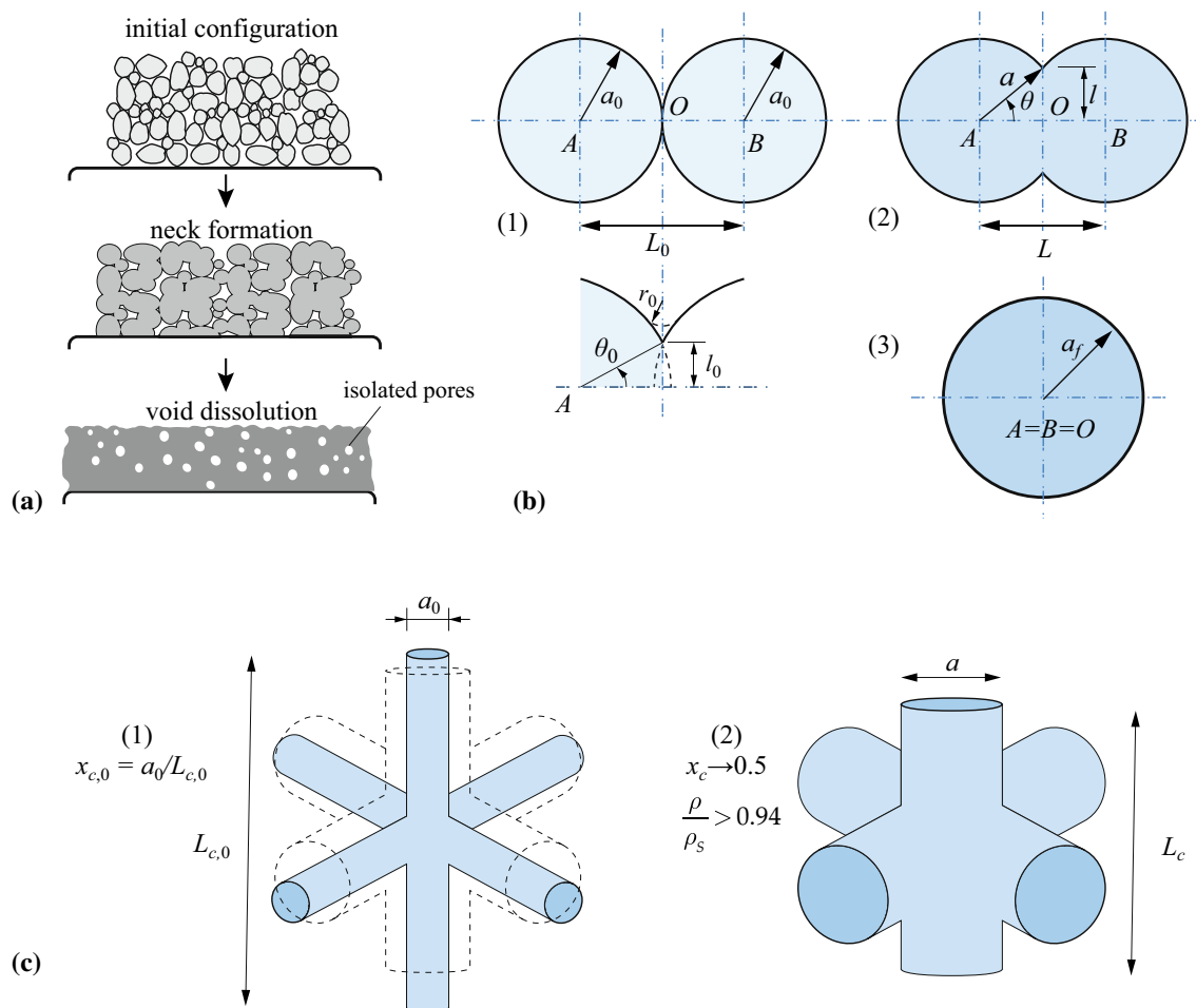
Figure 7 a Two-dimensional scheme of the densification process in a polymeric powder bed. b Frenkel's model describing the coalescence of two spherical particles [110]. c Scherer's model [117].
