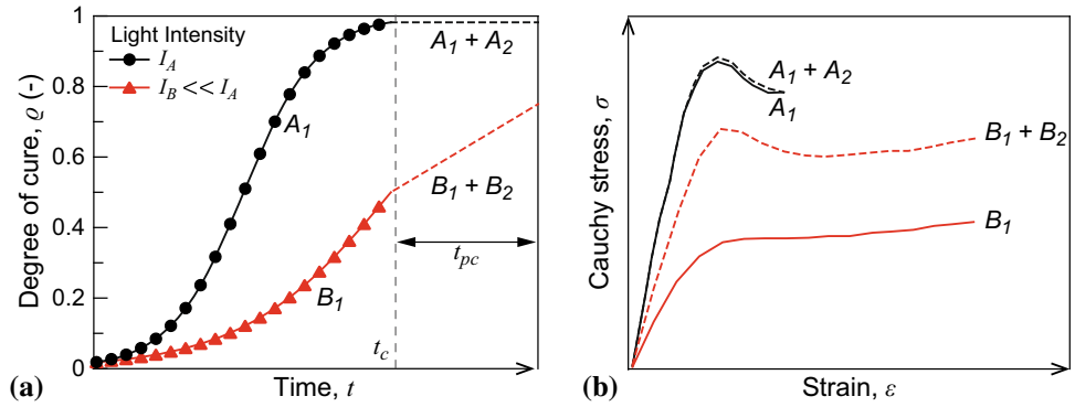
Figure 20 Schematic view of the effect of post-curing on the degree of cure a and on the mechanical behaviour of a component, before and after post-curing time b .
