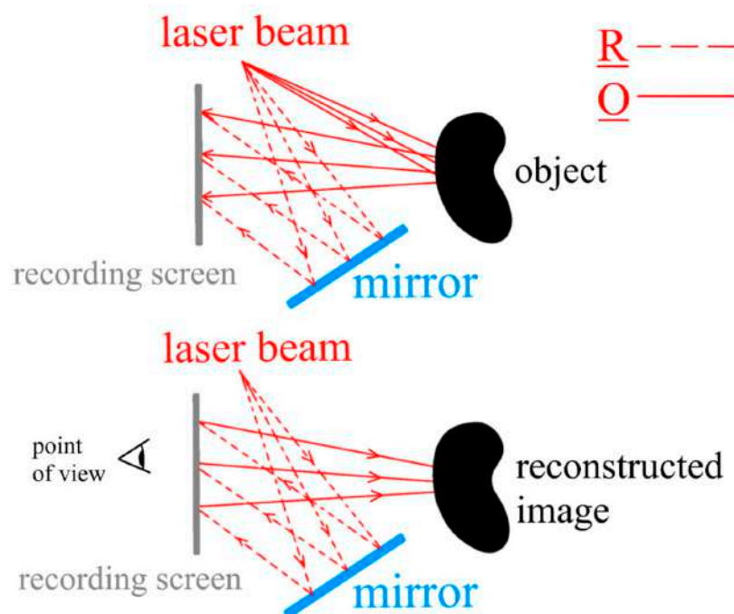
Figure 36. Holography working principle.
