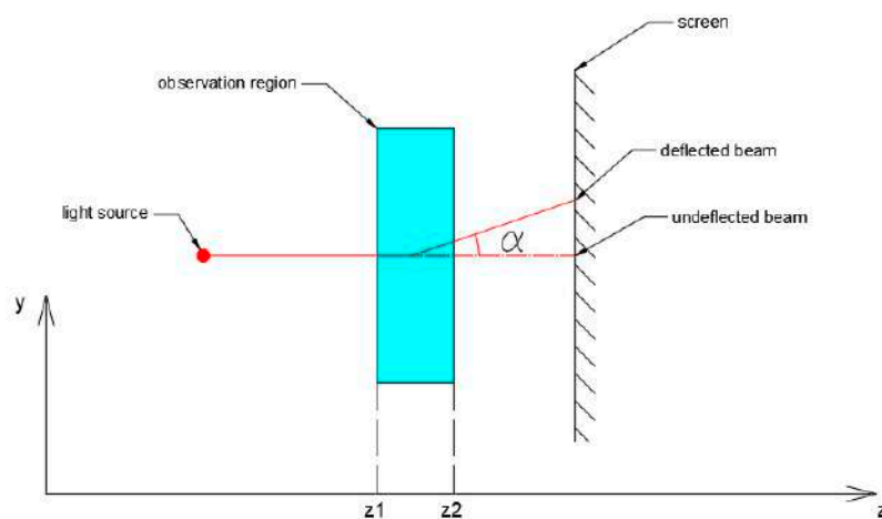
Figure 11. Shadowgraph principle.
