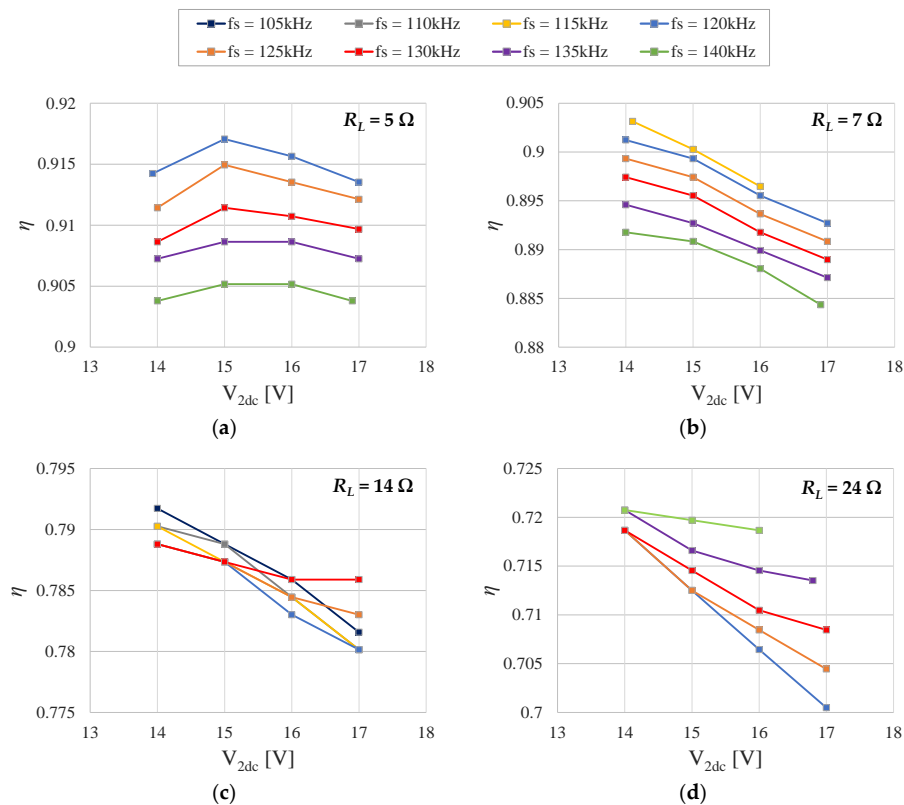
Figure 25. Experimental PR-IPTS efficiency vs. intermediate bus voltage V_{2dc} and inverter switching frequency f_s for different load conditions: (a) R_L = 5 \Omega ; (b) R_L = 7 \Omega ; (c) R_L = 14 \Omega ; and (d) R_L = 24 \Omega .
