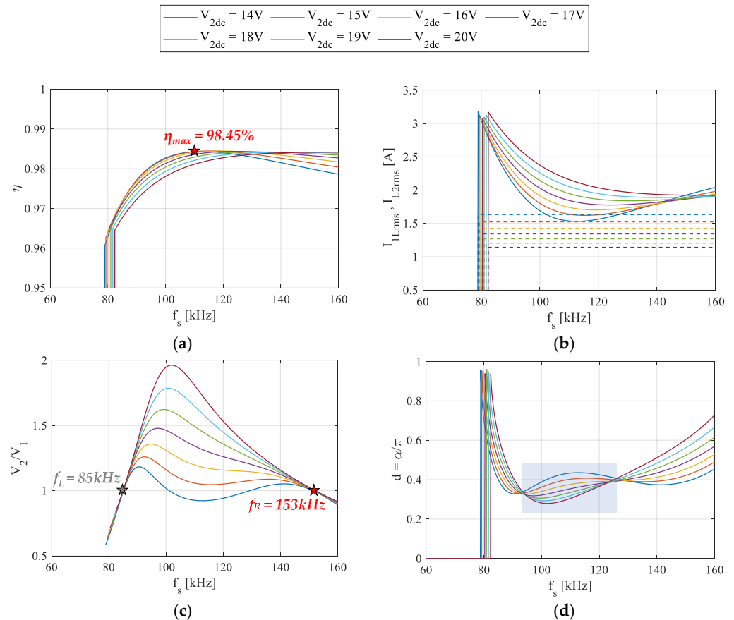
Figure 12. Predictions of IPTS modeling solution (5)–(8) vs. f_s for different values of V_{2dc} , for the capacitor set-up \{C_1 = 100 \text{ nF}, C_2 = 100 \text{ nF}\} : (a) IPTS efficiency \eta ; (b) TX and RX coil rms currents I_{L1rms} (solid), I_{L2rms} (dashed); (c) IPTS RX-to-TX voltage gain V_2/V_1 ; and (d) normalized phase-shift d .
