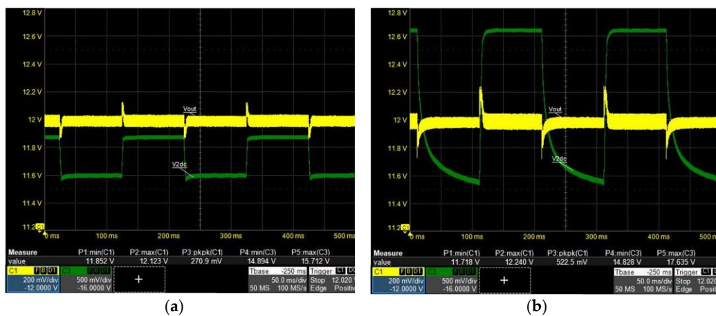
Figure 28. Experimental waveforms of v_o(t) (yellow) and v_{2dc}(t) (green) at f_s = 120 kHz and f_{LT} = 5 Hz for different load transient conditions: (a) R_L = \{7-14\} \Omega ; and (b) R_L = \{5-24\} \Omega .
