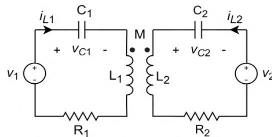
Figure 15. AC equivalent circuit of the IPT stage.
