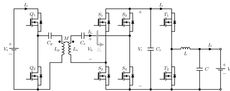
Figure 4. S-S IPTS with active rectifier and buck post-regulator [18].
