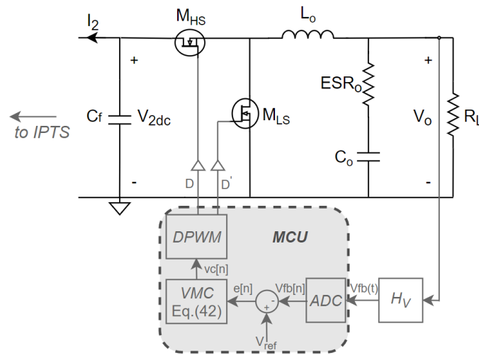
Figure 19. DVMC of the buck converter.
