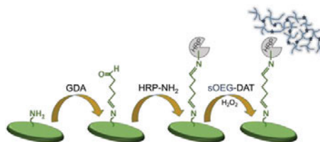
Fig. 1: Scheme of steps for surface functionalization and vision of enzyme-catalyzed thin layer hydrogel coating. The immobilized HRP should convert DAT moieties into corresponding phenoxyl radicals, which are further reacting to form covalent netpoints (stars) connecting several oligoethylene arms. A color version of the figure is available online.
