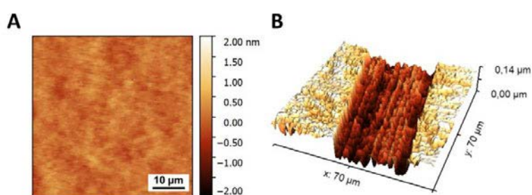
Fig. 5: Characterization of sample surfaces by AFM in aqueous environment. (A) Homogeneous topography of sample surface. (B) Micrograph of a scratch on sample surface used for determination of coating layer thickness.
