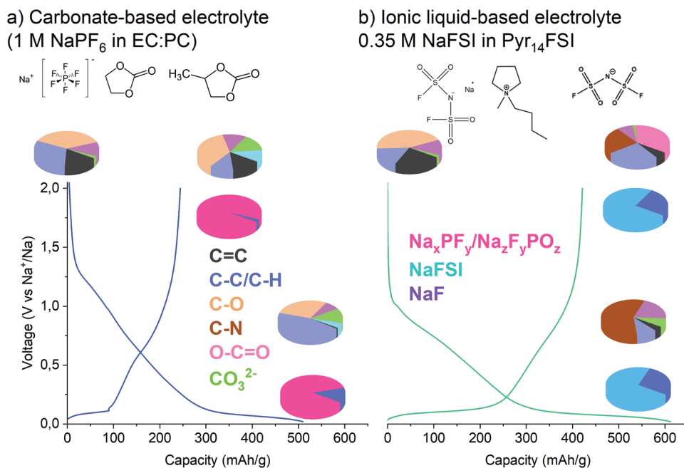
Figure 7. Voltage profile of the 1st cycle and the concentration of the SEI species obtained by fitting C 1s and F 1s photoelectron lines of hard carbon negative electrode tested in a) carbonate ester-based (1M NaPF 6 in EC:PC) and b) ionic-liquid (0.35M Na[FSI] in [Pyr 14 ][FSI]) electrolyte.
