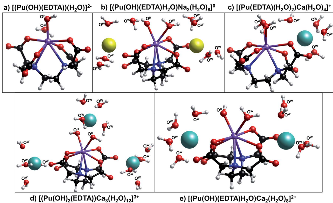
Fig. 6 Ball-and-stick models of the DFT optimized structures (a) [\text{Pu}(\text{OH})(\text{EDTA})(\text{H}_2\text{O})]^{2-} , (b) [\text{Pu}(\text{OH})(\text{EDTA})\text{H}_2\text{O}\text{Na}_2(\text{H}_2\text{O})_8]^0 , (c) [(\text{Pu}(\text{EDTA})(\text{H}_2\text{O})_2)\text{Ca}(\text{H}_2\text{O})_4]^+ , (d) [(\text{Pu}(\text{OH})_2(\text{EDTA}))\text{Ca}_3(\text{H}_2\text{O})_{12}]^{3+} , and (e) [(\text{Pu}(\text{OH})(\text{EDTA})\text{H}_2\text{O})\text{Ca}_2(\text{H}_2\text{O})_8]^{2+} calculated at the hybrid density functional theory level (B3LYP). Water and hydroxyl oxygen atoms are labeled with \text{O}^{\text{W}} and \text{O}^{\text{H}} , respectively, while carboxyl oxygen atoms within the EDTA ligand are unlabeled. Legend: plutonium (purple), sodium (yellow), calcium (light blue), carbon (black), oxygen (red), nitrogen (dark blue), and hydrogen (white).
