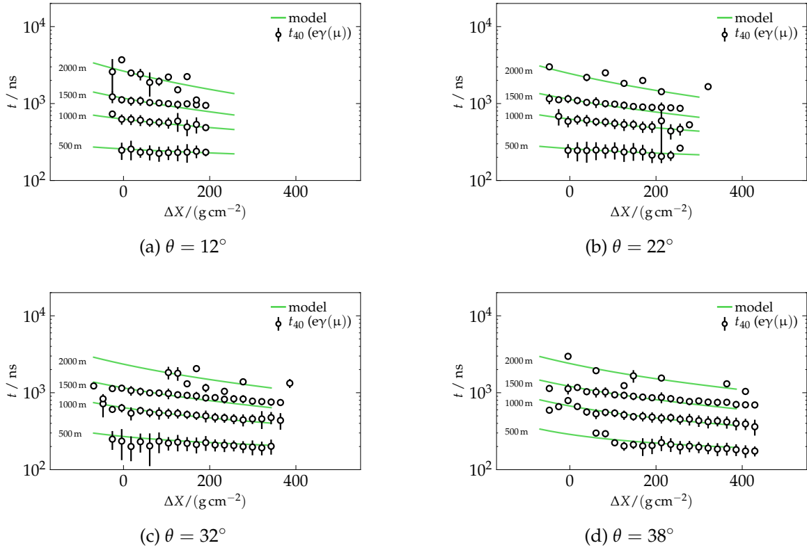
Figure B.9: Values of t_{40} for the e\gamma(\mu) component as a function of \Delta X obtained from WCD responses to showers of E_0 = 10^{19} eV and 10^{20} eV and various zenith angles, alongside with the model resulting from the parametrization.
