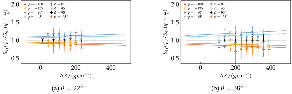
Figure 5.17: Asymmetry in azimuth for the signals of the e\gamma component from showers of E_0 = 10^{19} eV deposited in WCDs at r = 750 m for (a) \theta = 22^\circ and (b) \theta = 38^\circ . Upstream regions are colored in blue, downstream regions are colored in orange.
