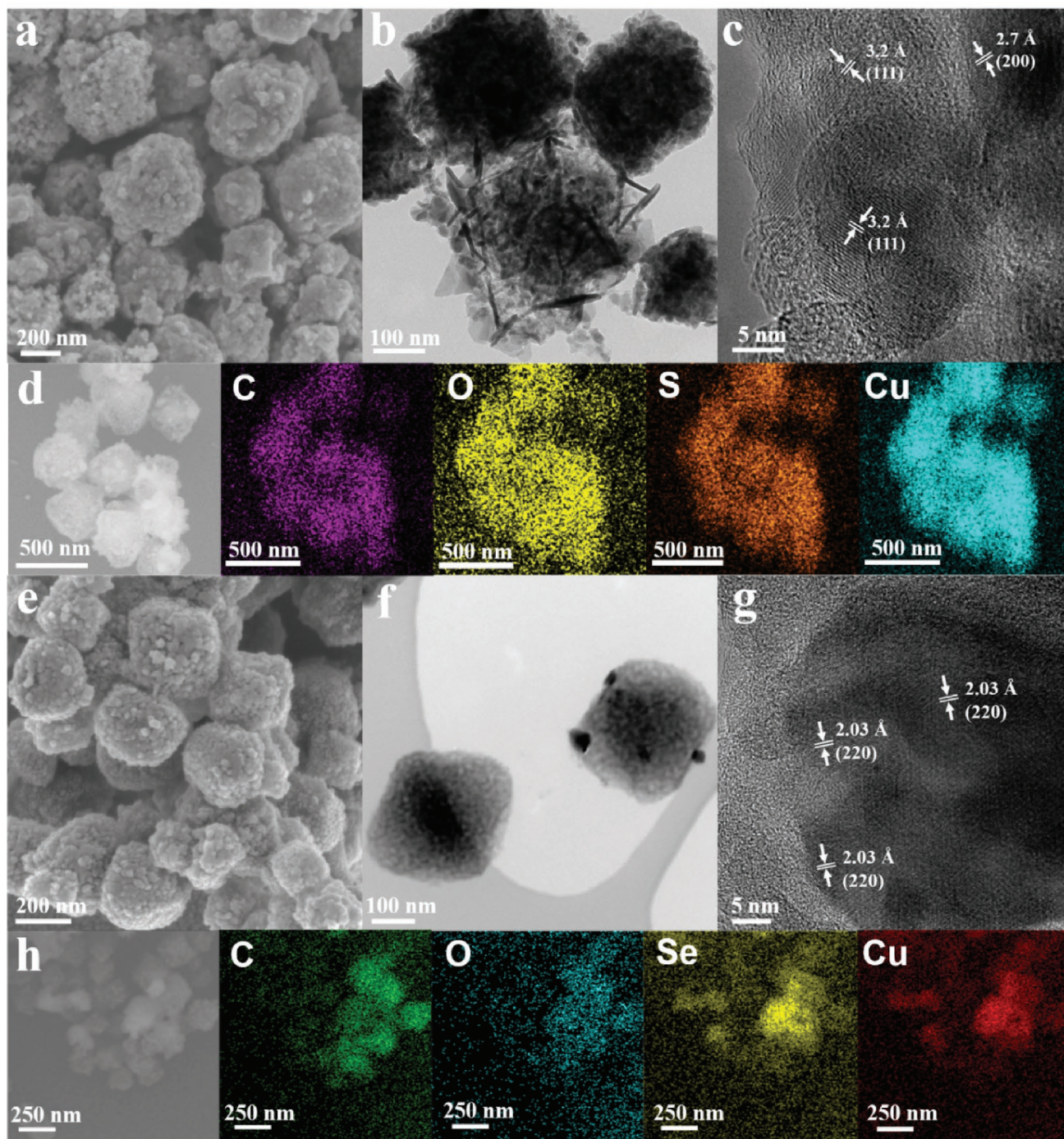
Figure 3. Morphological and structural features of Cu 1.8 S@C and Cu 2-x Se@C. a) SEM, b,c) HR-TEM, and d) Elemental mapping images of Cu 1.8 S@C. e) SEM, f,g) HR-TEM, and h) Elemental mapping images of Cu 2-x Se@C.
