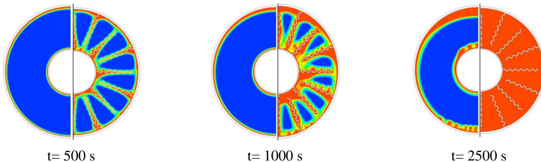
Figure 4: Liquid fraction contours at 500s, 1000s, and 2500s of flow time comparing the base design (left) against the long-length waved fin design (right).
