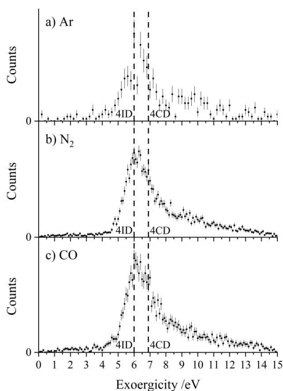
Figure 3: Experimental exoergicities resulting from the CID channel \text{CH}_2\text{CN}^{2+} + \text{X} \rightarrow \text{CH}_2\text{N}^+ + \text{C}^+ + \text{X} , where \text{X} = \text{a) Ar, b) N}_2 , and \text{c) CO} . Dashed lines are marked at 6.0 eV and 6.9 eV in each of the distributions to show the predicted literature exoergicities associated with the involvement of the quartet linear isocyanide dication 4ID and the cyclic quartet dication 4CD respectively. The error bars represent two standard deviations of the counts.
