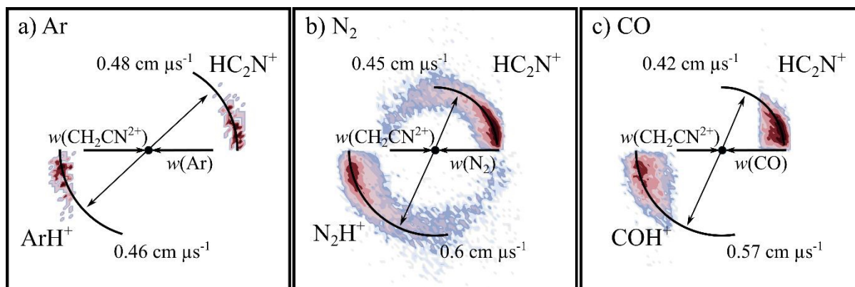
Figure 5: CM scattering diagrams for the PT channel CH_2CN^{2+} + X \rightarrow HC_2N^+ + XH^+ . a) X = Ar at a CM collision energy of 5.0 eV, b) X = N_2 at a CM collision energy of 4.5 eV, and c) X = CO at a CM collision energy of 4.3 eV.
