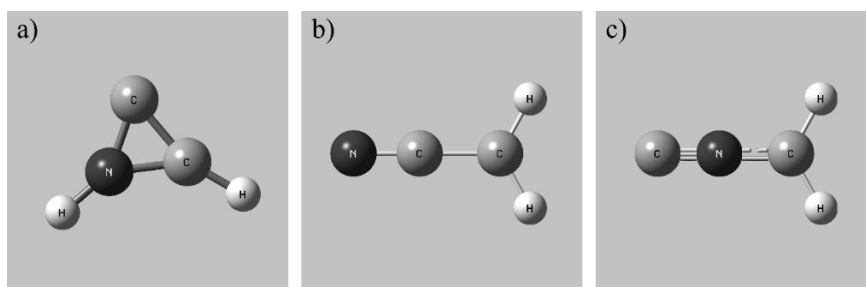
Figure 1: Geometries of the local minima of the reactant \text{CH}_2\text{CN}^{2+} dication (doublet states). a) cyclic conformation, 2CD, b) linear conformation, 2LD, c) linear isocyanide conformation, 2ID. See text for details.
