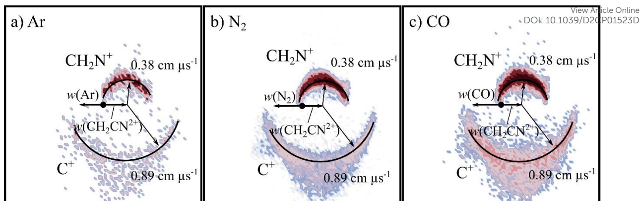
Figure 2: CM scattering diagrams for the CID channel producing \text{CH}_2\text{N}^+ + \text{C}^+ resulting from the reactions of a) \text{CH}_2\text{CN}^{2+} + \text{Ar} at a CM collision energy of 5.0 eV, b) \text{CH}_2\text{CN}^{2+} + \text{N}_2 at a CM collision energy of 4.5 eV, and c) \text{CH}_2\text{CN}^{2+} + \text{CO} at a CM collision energy of 4.3 eV.
