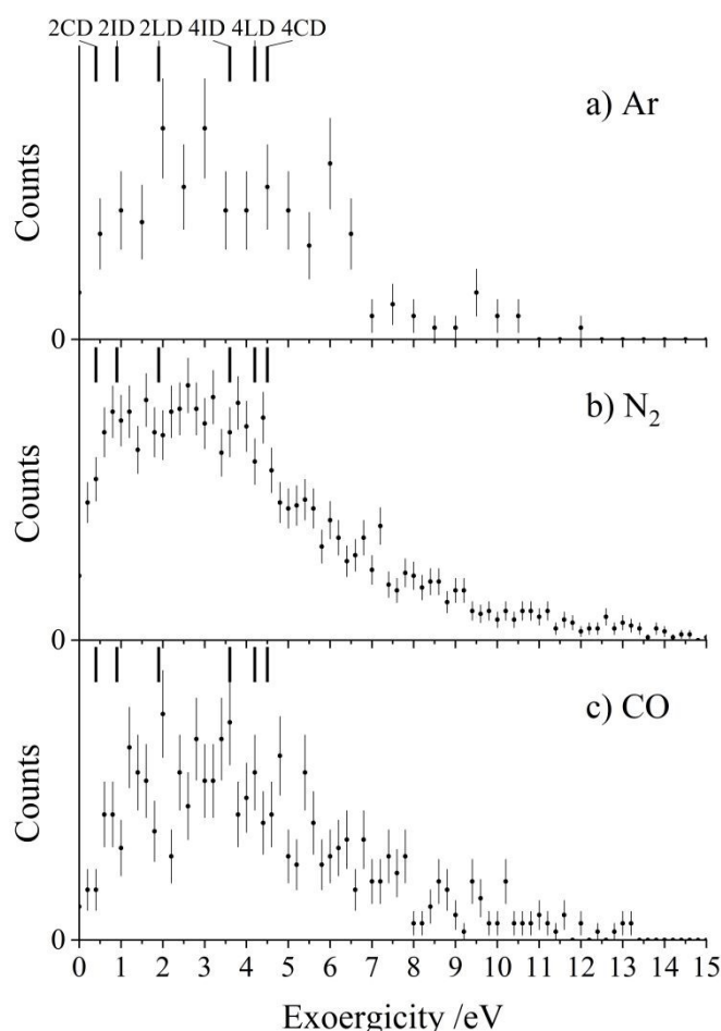
Figure 4: Experimental exoergicity distributions resulting from the channel \text{CH}_2\text{CN}^{2+} + \text{X} \rightarrow \text{HC}_2\text{N}^+ + \text{H}^+ + \text{X} , where \text{X} = \text{a) Ar, b) N}_2 , and c) \text{CO} . Lines are marked in each of the distributions to show the literature exoergicities for reactions involving each of the six dication states. The error bars represent two standard deviations of the counts.
