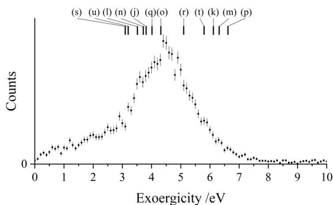
Figure 9: Experimental exoergicity distributions resulting from the NDSET reaction between \text{CH}_2\text{CN}^{2+} + \text{CO} , resulting in the formation of \text{CH}_2\text{CN}^+ + \text{CO}^+ . The literature exoergicities resulting from pathways (j) – (u) are marked, see Table 7 for details. The error bars represent two standard deviations of the counts.
