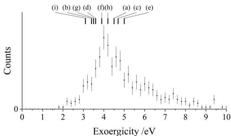
Figure 8: Experimental exoergicity distributions resulting from the NDSET reaction between \text{CH}_2\text{CN}^{2+} + \text{N}_2 , resulting in the formation of \text{CH}_2\text{CN}^+ + \text{N}_2^+ . The literature exoergicities resulting from pathways (a) – (i) are marked, see Table 6 for details. The error bars represent two standard deviations of the counts.
