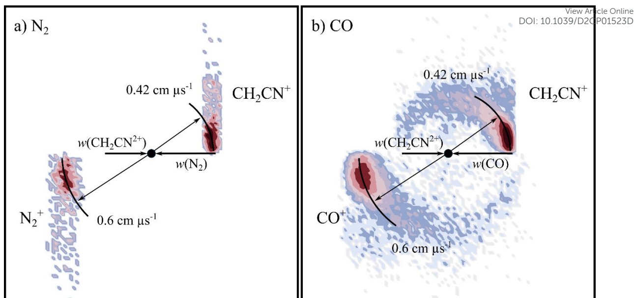
Figure 7: CM scattering diagrams for the NDSET channel \text{CH}_2\text{CN}^{2+} + \text{X} \rightarrow \text{CH}_2\text{CN}^+ + \text{X}^+ . a) \text{X} = \text{N}_2 at a CM collision energy of 4.5 eV b) \text{X} = \text{CO} at a CM collision energy of 4.3 eV.
