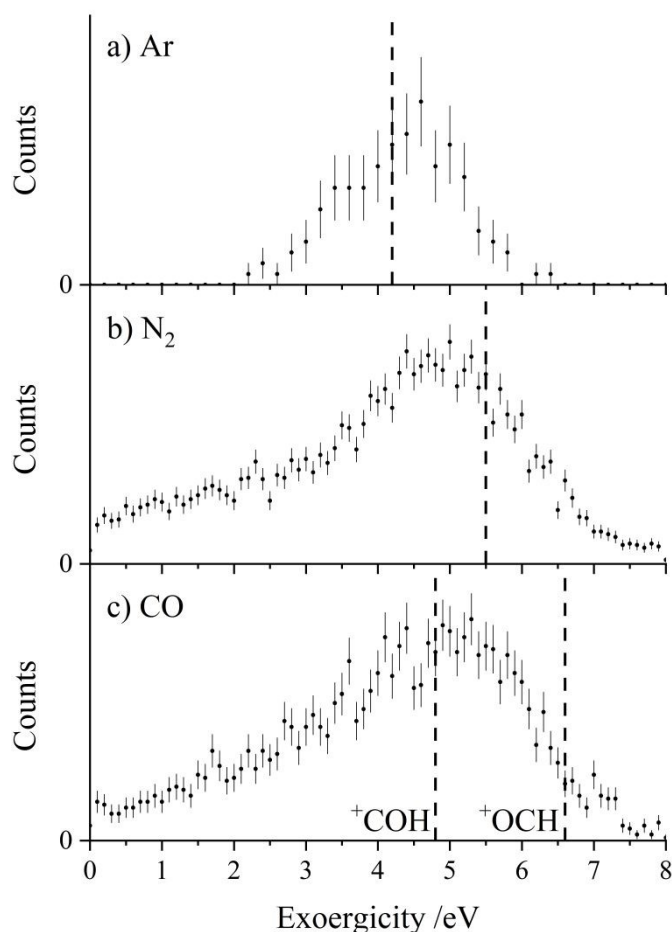
Figure 6: Experimental exoergicity distributions resulting from the PT reactions \text{CH}_2\text{CN}^{2+} + \text{X} \rightarrow \text{HC}_2\text{N}^+ + \text{XH}^+ . a) \text{X} = \text{Ar} , b) \text{X} = \text{N}_2 , c) \text{X} = \text{CO} . Lines are marked on each distribution corresponding to the expected literature exoergicity from forming \text{XH}^+ + \text{HC}_2\text{N}^+ in their ground states from the ground state dication, 2CD. For CO, there are two possible \text{XH}^+ products, \text{COH}^+ and \text{OCH}^+ . The error bars represent two standard deviations of the counts.
