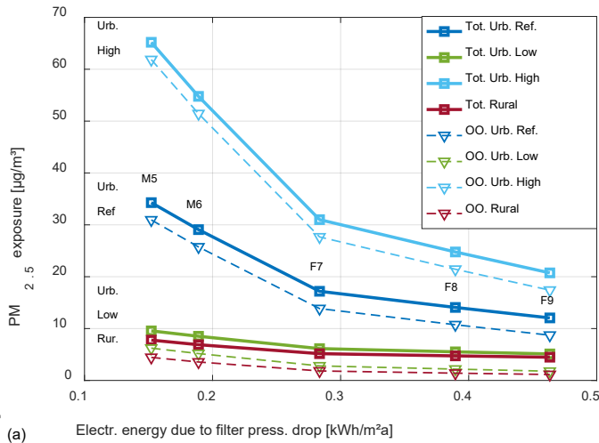
Figure 3-9 Average PM 2.5 exposure of a person staying home all day as a function of electric energy consumption of the fan due to the pressure drop of the filter. “Urb. High” represents highly polluted areas with daily means of ~80 µg/m 3 , “Urb. Ref” moderately polluted areas with means of ~40 µg/m 3 and “Urb. Low” low polluted urban areas with a daily mean ~8 µg/m 3 . The dashed line/triangle show the exposure to outdoor-originate PM.
