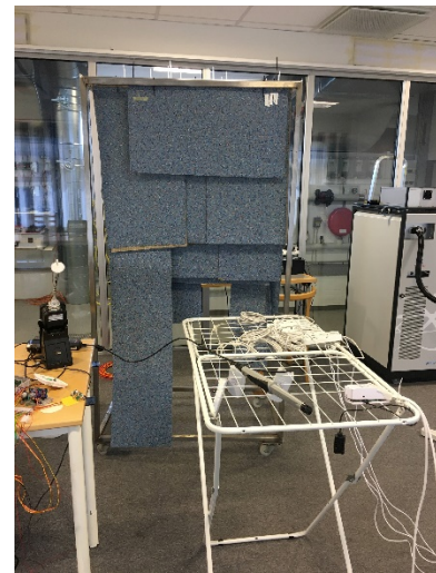
Figure 3-20 Experimental set-up with sensors and linoleum as a pollution source.
