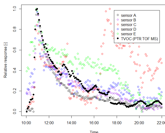
Figure 3-22 Activity: cleaning with detergent; normalized MOS VOC signals compared with TVOC PTR-TOF-MS .
