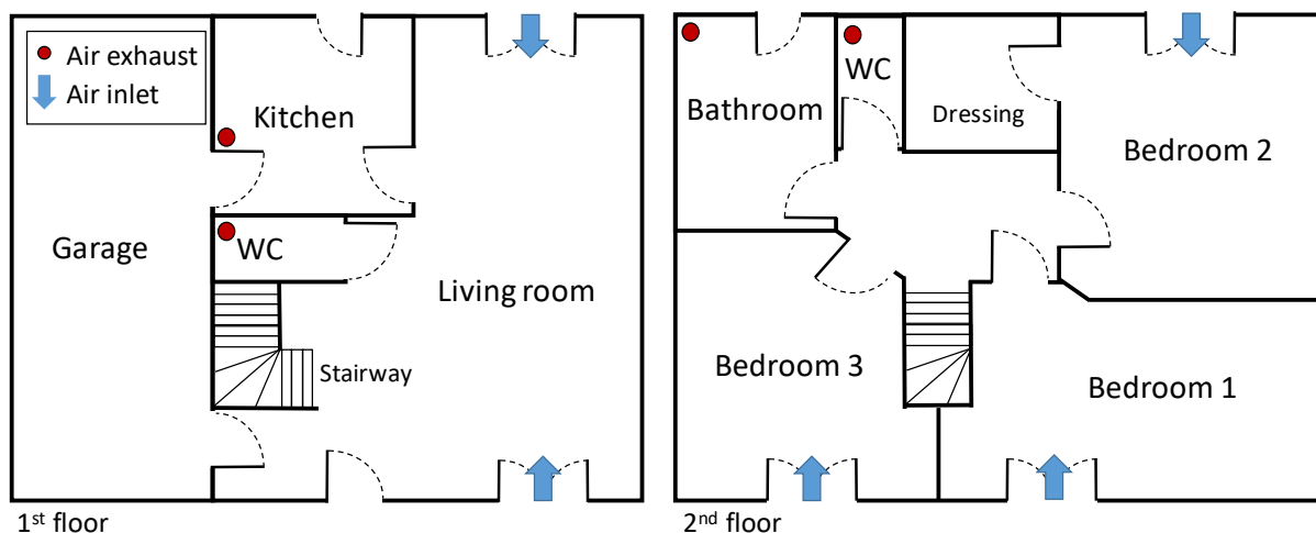
Figure 4-54 Building design.
