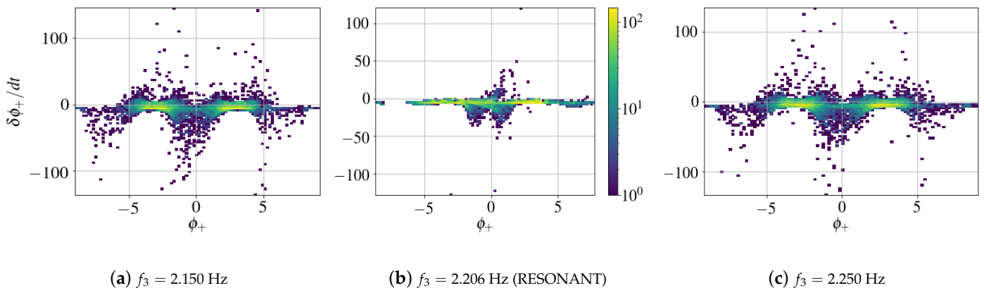
Figure 7. Joint probability density functions of the quintet phase \phi_+(t) versus its time derivative \frac{d\phi_+}{dt}(t) , over the simulation time t \in [0, 200 \text{ s}] , for the cases f_3/\text{Hz} = 2.150, 2.206 and 2.250 in the plane-wave case, corresponding to Figures 3 and 5.
