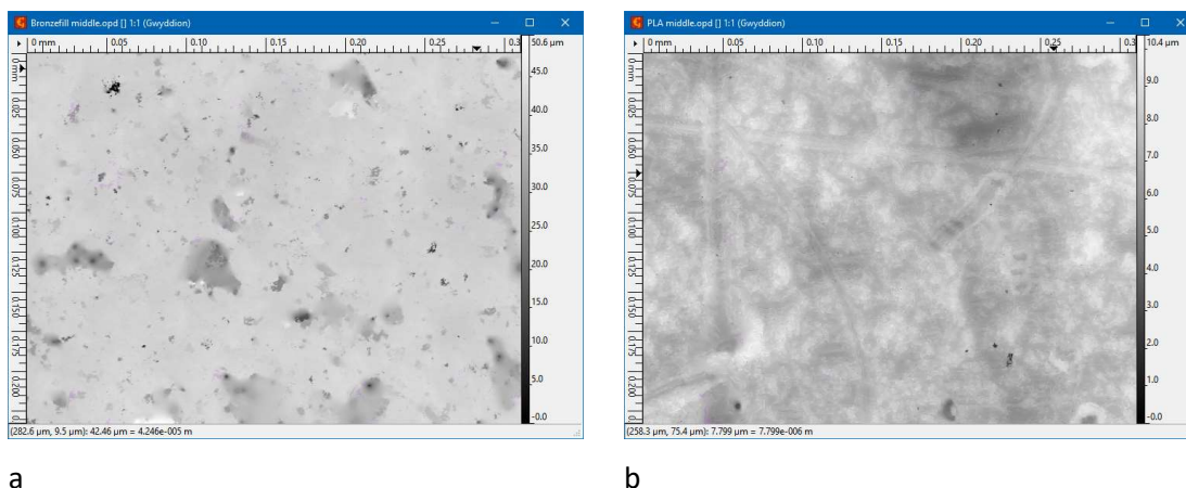
Figure 4-8: a - Bronzefil (height colour scale: 0 – 50 µm), b - PLA (height colour scale: 0 - 10.4 µm), both on PEI, illustrating variation in maximum height between materials.
