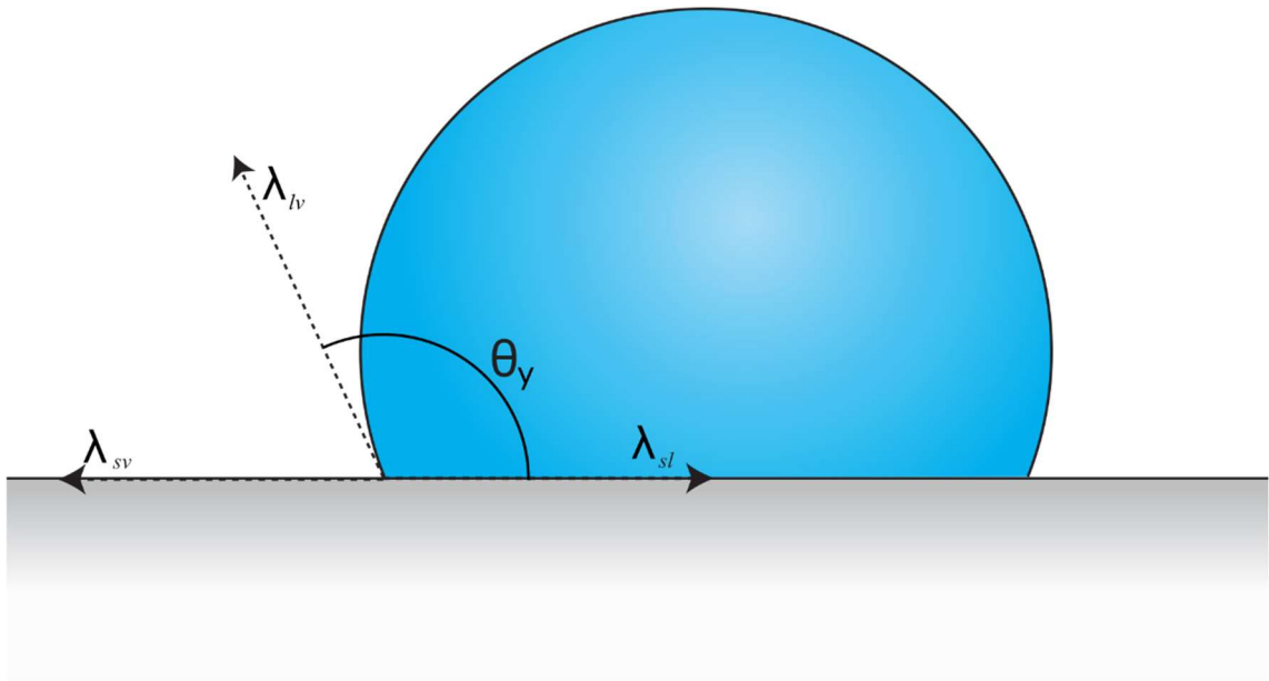
Figure 2-21: Illustration of contact angles with surface energies
