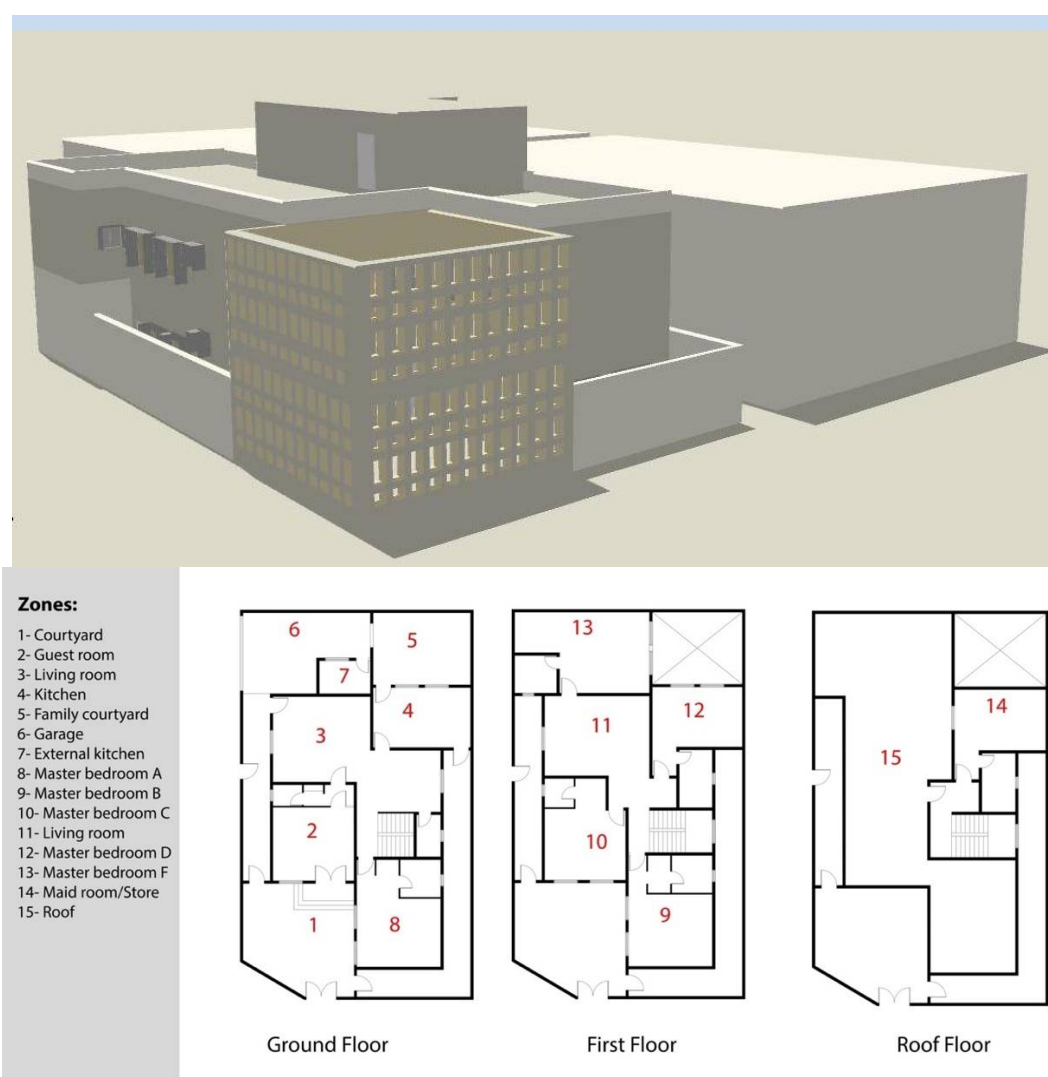
Figure 15. The prototype 3D model space distribution.
