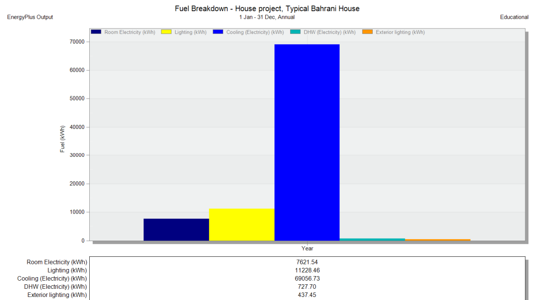
Figure 13. Breakdown of energy consumption in the case study house using air conditioning.
