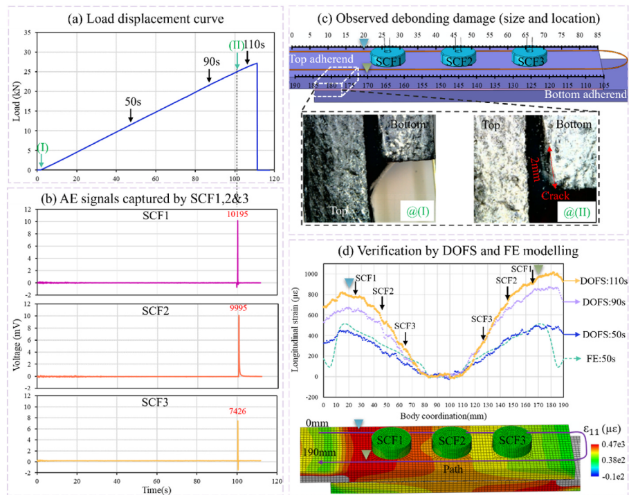
Fig. 5. Experiment and FE modelling results of type-C SLJ: (a) The load-displacement curve of the measured SLJ sample; (b) The AE signals captured by SCF 1,2 and 3; (c) The observations of sizes and locations of the debonding damages in the joint associated with the sample images; (d) The comparison of longitudinal strains measured from DOFS and FE modelling corresponded to the DOFS path.
