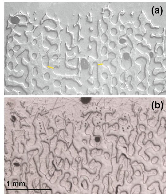
Fig. 4 Reflected light micrographs of cross sections through the outermost surface of coral genotype 7 cultured at a 400 μatm and b 750 μatm. Typical positions of trabeculae width measurements are shown by yellow lines. Ion microprobe analysis pits are visible as small black dots on the images
