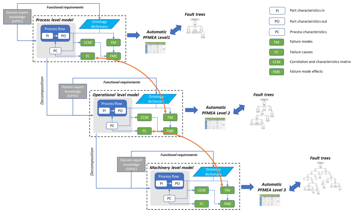
Figure 3. Generic methodology towards automatic PFMEA
