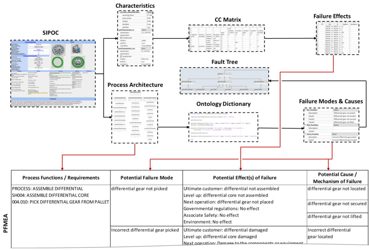
Figure 6. MBSE output information flow into PFMEA
