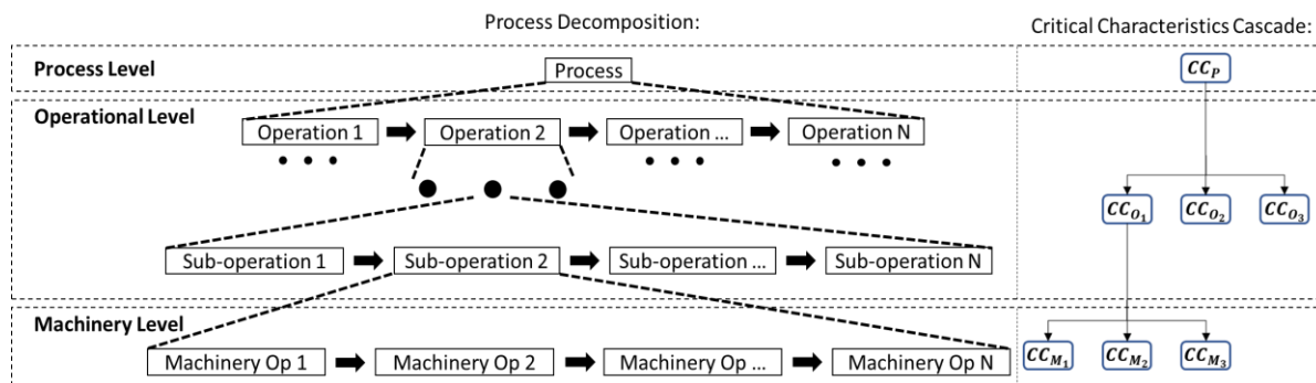
Figure 4. Top-down robotic manufacturing process decomposition
