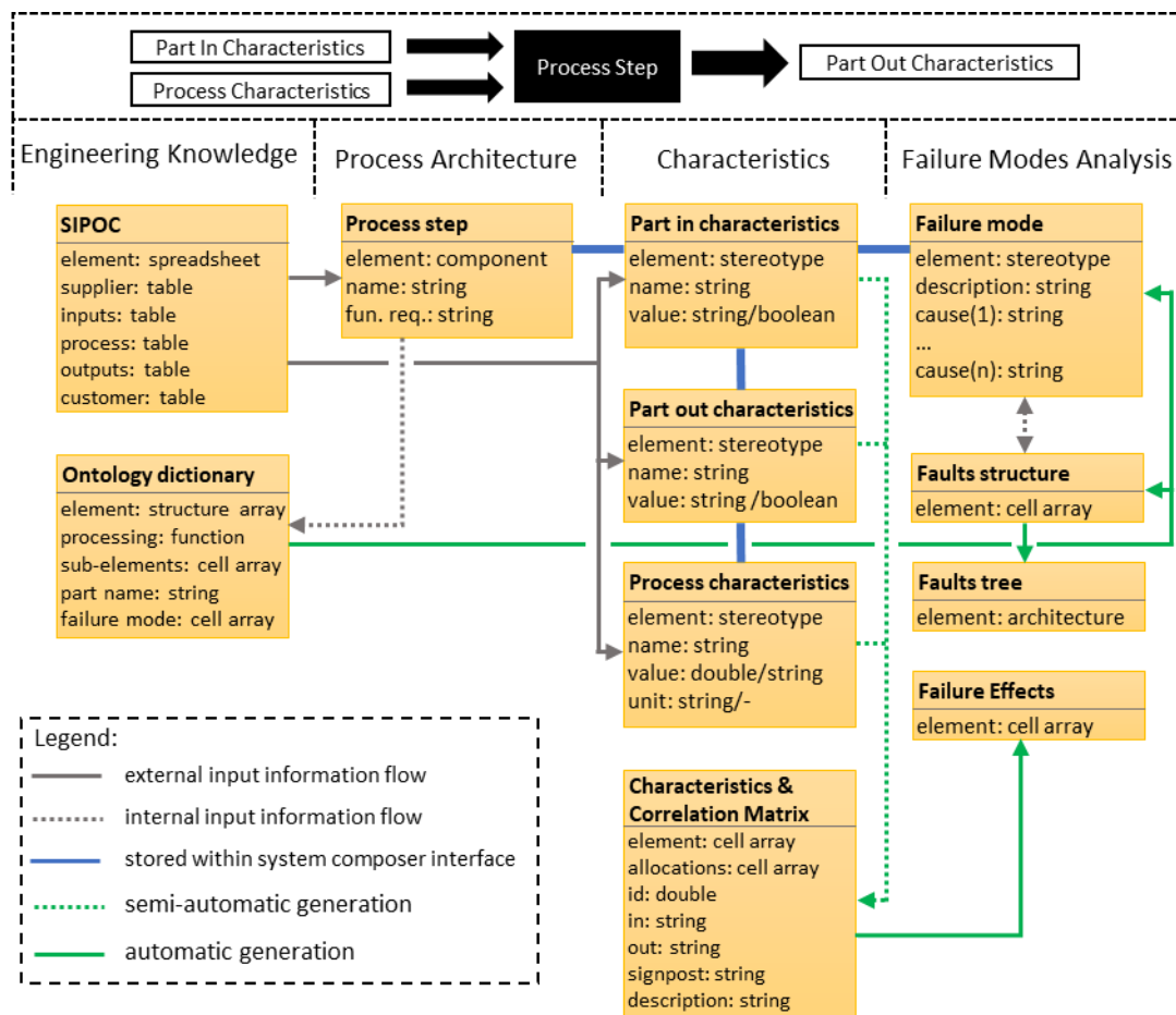
Figure 5. MBSE robotic manufacturing process model database structure
