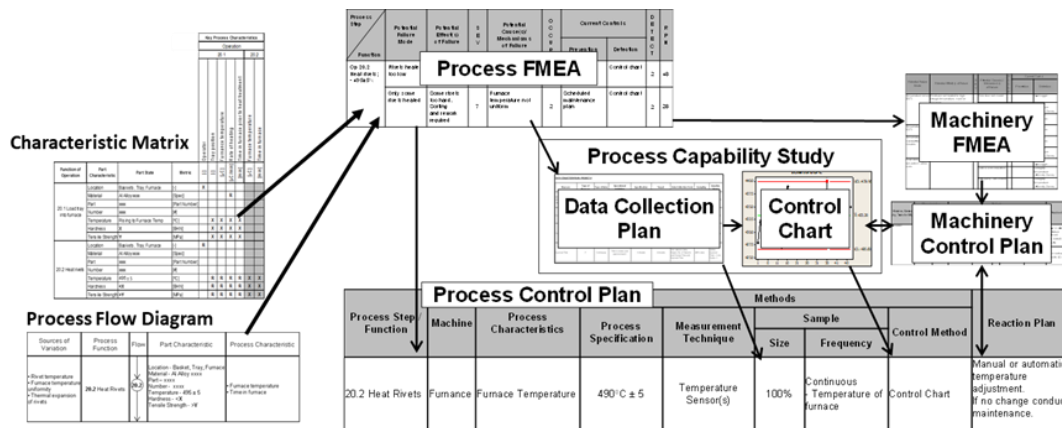
Figure 2. Integrated process FMEA with dynamic control planning
