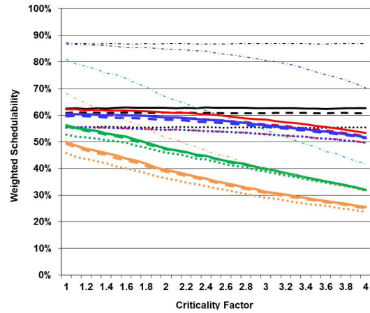
Figure 6: Weighted Schedulability: Varying the Criticality Factor, 2 cores.
