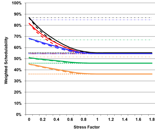
Figure 5: Weighted Schedulability: Varying Resource Stress, 2 cores.
