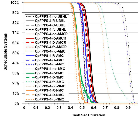
Figure 4: Success Ratio: Varying task set utilization, 4 cores.
