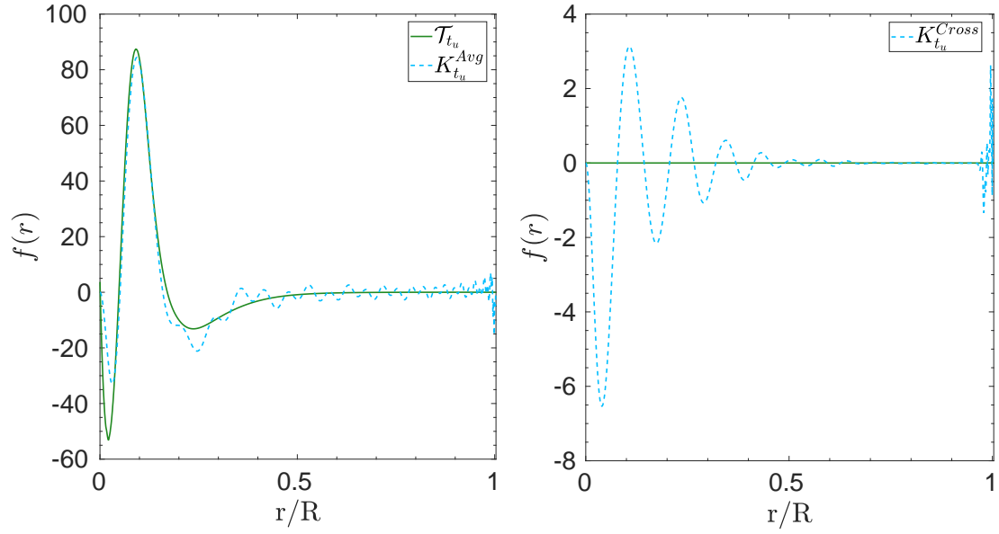
Fig. A.5. Averaging kernel for the t_u inversion of 16CygA (left, blue) and its associated target function (green). Cross-term kernel for the t_u inversion of 16CygA (right, blue) and its associated target function (green).
