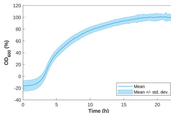
Fig. 2 Growth curve of P. aeruginosa over 24 hours. Y axis shows optical density measured at 600 nm, normalised against the negative control (LB only). Note that growth reaches a stationary phase at ~15 hours.
