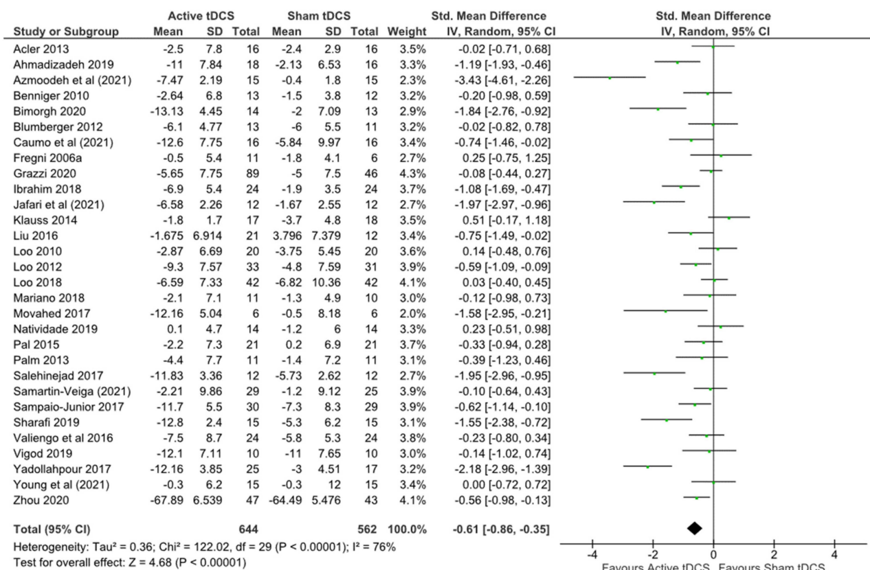
Figure 4. Forest plot depression.
