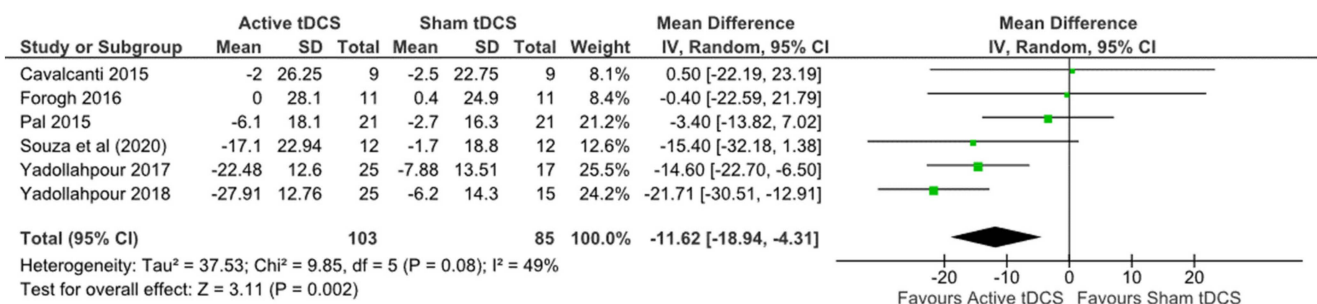
Figure 3. Forest plot tinnitus.
