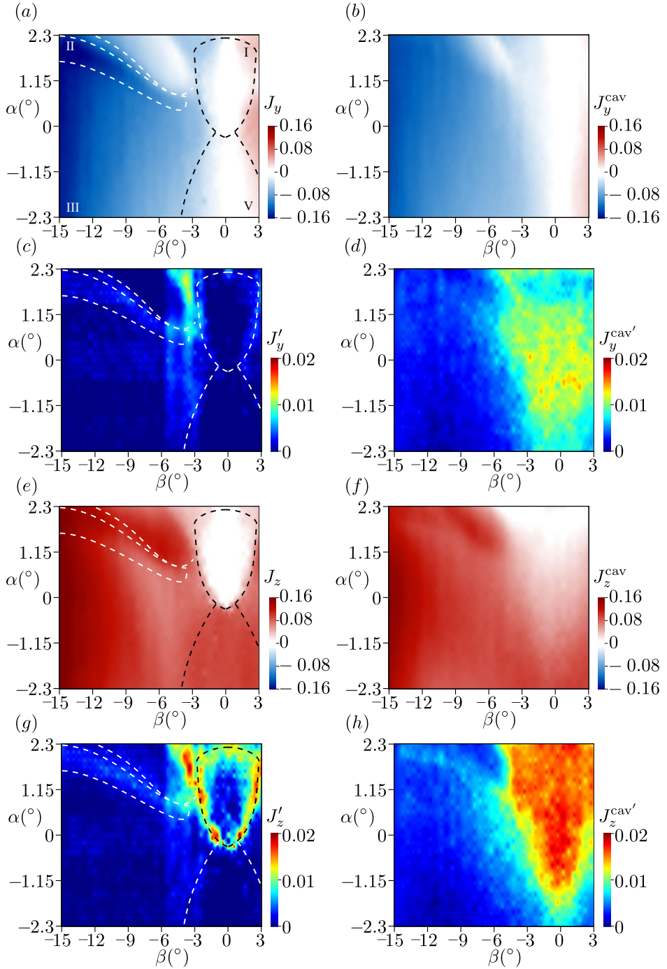
FIGURE 16. Components of the mean \mathbf{J}(\beta, C_0^* = 0.1, \alpha) (a, e) and fluctuating \mathbf{J}'(\beta, C_0^* = 0.1, \alpha) (c, g) pressure gradient at the rear of the body lateral surfaces. Case with the rear cavity : \mathbf{J}^{\text{cav}}(\beta, C_0^* = 0.1, \alpha) (b, f) and \mathbf{J}^{\text{cav}' }(\beta, C_0^* = 0.1, \alpha) (d, h). The dashed lines in (a, c, e, g) are all transition lines reported from figure 10(b) with the regions labeling in (a). Colours are adapted for a better contrast.
