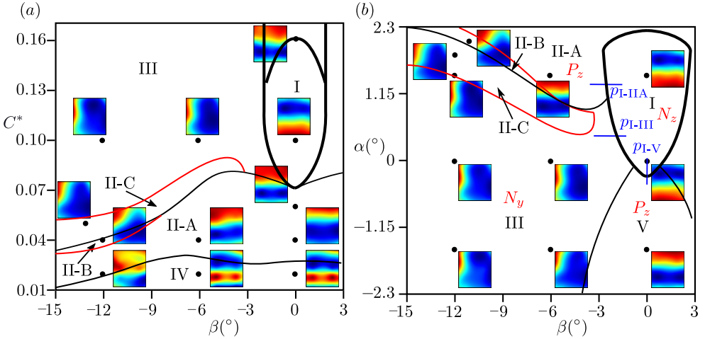
FIGURE 10. Recap of transitions for the clearance (a) and pitch (b) vs. yaw mappings deduced from figure 8 and figure 9. All lines are transitions in G_y and G_z reported from Fig. 8 where red (resp. black) lines are transitions for G_y (resp. G_z ). Thick lines depict transitions associated with large base pressure gradient fluctuations. The color maps show the representative base pressure distribution in different regions, with an autoscale color bar, the red (resp. blue) indicates high (low) pressure. The three blue paths in (b) denote the unsteady transitions investigated in §3.4.
