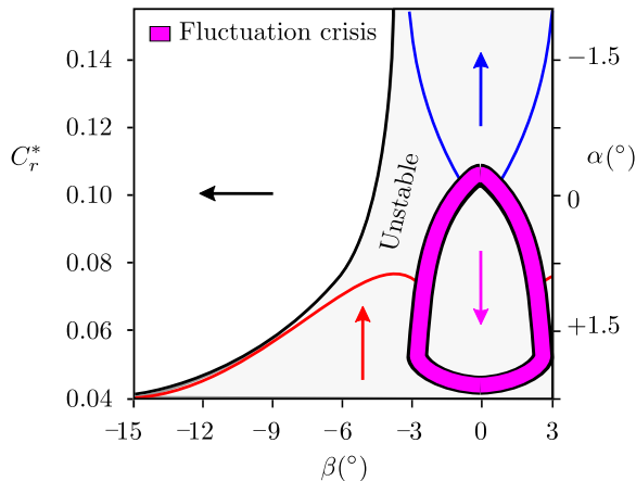
FIGURE 18. Z -instability domain of the wake as a function of the body attitude (defined by yaw \beta and pitch \alpha or rear clearance C_r^* ) deduced from the rear cavity experiment and transitions in the base pressure gradient. The orientation of the pressure gradient is indicated with arrows.
