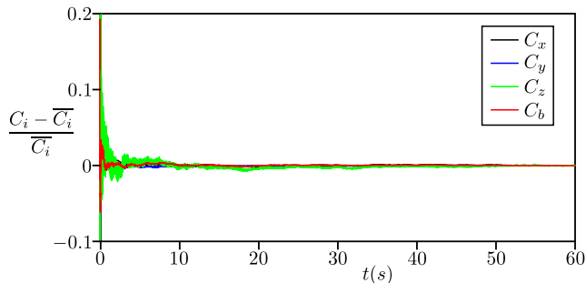
FIGURE 2. Convergence of the average coefficient of the force components and base suction at the reference attitude.
