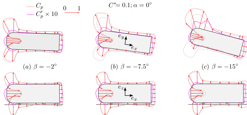
FIGURE 4. Same caption as for figure 3 except that the 3 cases (a, b, c) depict variations with different yaws with no pitch \alpha = 0^\circ and C^* = 0.1 .
