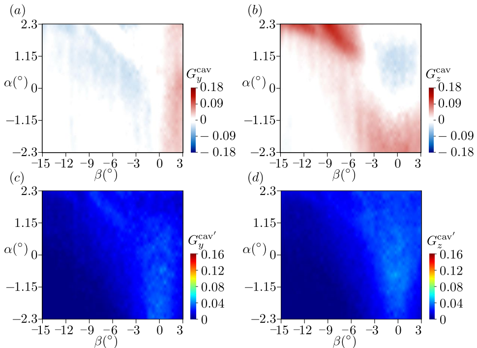
FIGURE 15. Case with the rear cavity: components of the mean \mathbf{G}(\beta, C_0^* = 0.1, \alpha) (a, b) and fluctuating \mathbf{G}'(\beta, C_0^* = 0.1, \alpha) (c, d) base pressure gradient for the pitch vs. yaw mapping.
