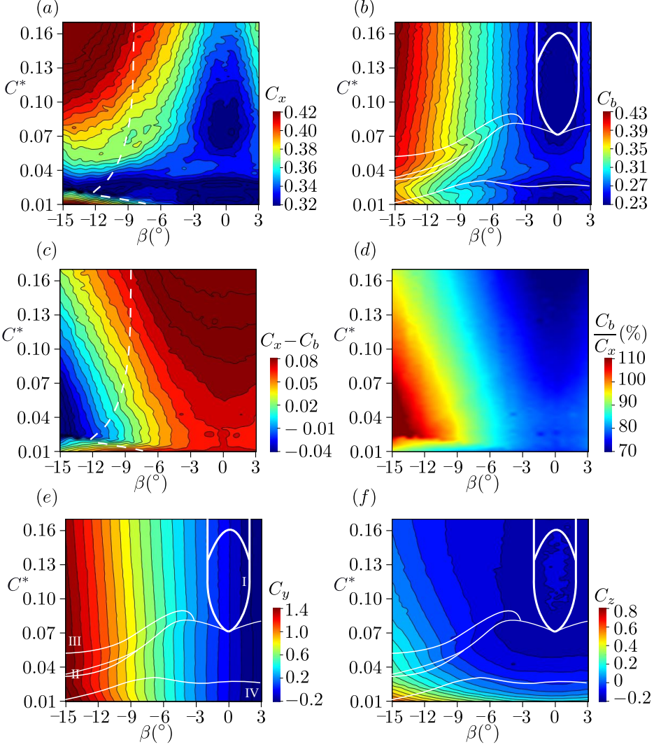
FIGURE 13. Force coefficient components for the clearance vs. yaw mapping ( \beta, C^*, \alpha_0 = 0^\circ ): (a) total drag coefficient C_x ; (b) base suction C_b ; (c) remainder drag except for the base suction C_x - C_b ; (d) base suction contribution to the total drag C_b/C_x (e) side force coefficient C_y ; (f) lift coefficient C_z . Dashed lines in (a, c) are the leeward separation lines as defined in Fig. 7(a). All lines in (b, e, f) are reported from Fig. 10(a) with thick lines for transitions associated with large base pressure gradient fluctuations. Regions are labeled in (e) as defined in figure 10.
