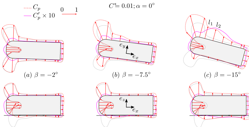
FIGURE 5. Same caption as for figure 3 except that the 3 cases (a, b, c) depict variations with different yaws with no pitch \alpha = 0^\circ and C^* = 0.01 .
