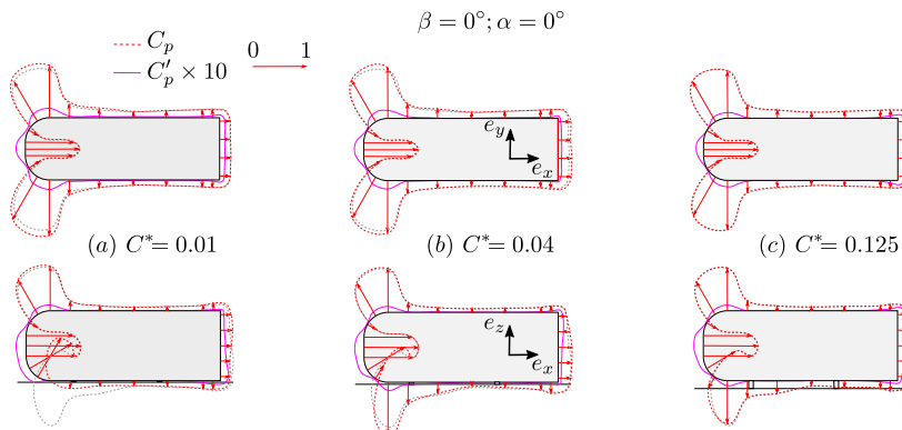
FIGURE 3. Mean ( C_p ) and fluctuating ( C'_p ) pressure coefficient distribution around the horizontal (top row) and vertical (bottom row) central sections of the body. The local pressure C_p is represented by red arrows, negative when pointed outward the body surface. C'_p is shown as the magenta continuous line. The grey dashed line is the C_p distribution at the baseline attitude \beta = \alpha = 0^\circ and C^* = 0.1 . The 3 cases (a, b, c) depict variations with different ground clearances and body aligned with the incoming flow ( \beta = \alpha = 0^\circ ).
