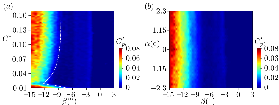
FIGURE 7. Regions of separation on the lateral leeward side for the variations of clearance and yaw (a) C'_{pl}(\beta, C^*, \alpha = 0^{\circ}) and pitch and yaw (b) C'_{pl}(\beta, \alpha, C^*_0 = 0.1) .
