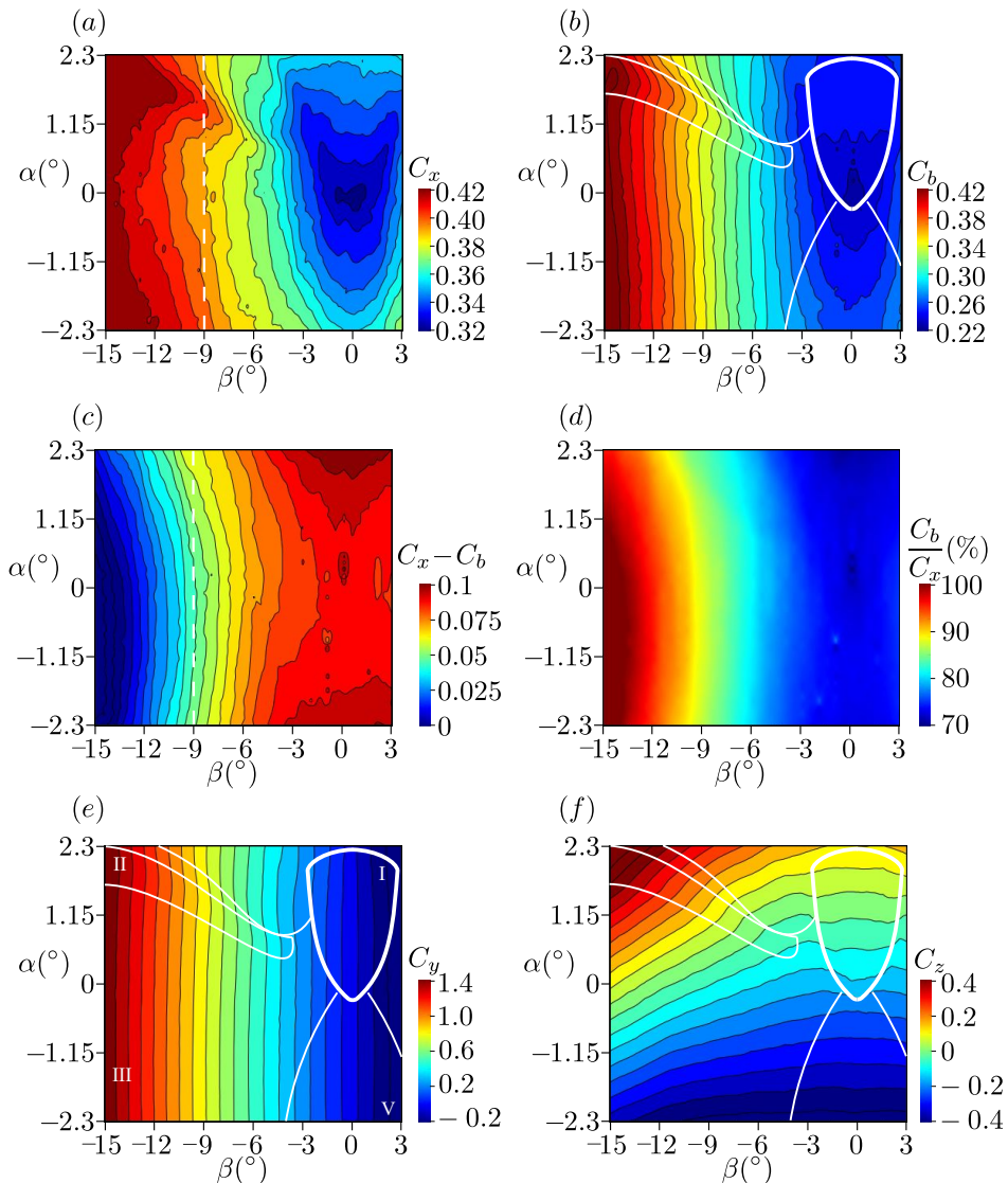
FIGURE 14. Force coefficient components for the pitch vs. yaw mapping ( \beta, C_0^* = 0.1, \alpha ): (a) total drag coefficient C_x ; (b) base suction C_b ; (c) remainder drag C_x - C_b except for the base suction C_x - C_b ; (d) base suction contribution to the total drag C_b/C_x (e) side force coefficient C_y ; (f) lift coefficient C_z . Dashed lines in (a, c) are the leeward separation lines as defined in Fig. 7(b). All lines in (b, e, f) are reported from Fig. 10(b) with thick lines for transitions associated with large base pressure gradient fluctuations. Regions are labeled in (e) as defined in figure 10.
