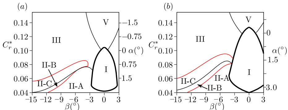
FIGURE 11. Recap of all transitions for the pitch vs. yaw maps represented in the (C_r^*, \beta) plane with (a) C_0^* = 0.1 reported from figure 10(b) and (b) C_0^* = 0.125 . The pitch \alpha equivalent to C_r^* is displayed as a second axis on the right hand side of the plots. Same legend for lines as in figure 10.
