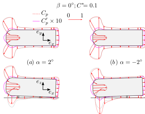
FIGURE 6. Same caption as for figure 3 except that the 2 cases (a, b) depict variations with different pitches with no yaw \beta = 0^\circ and C^* = 0.1 .
