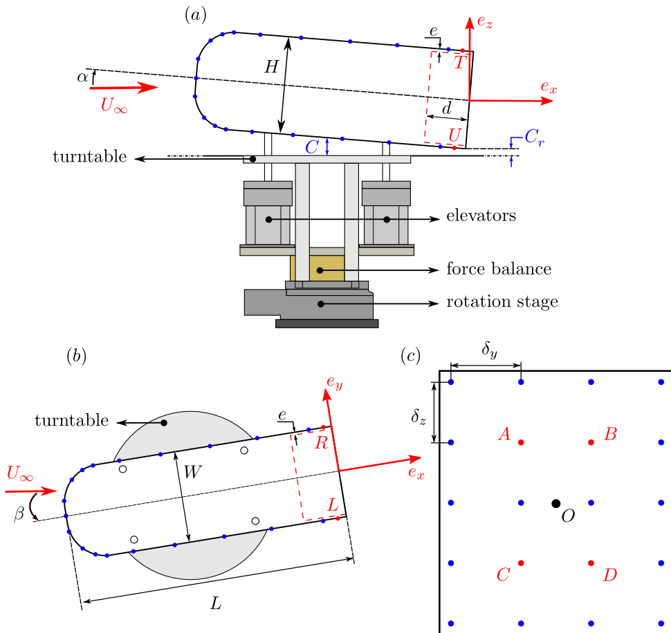
FIGURE 1. The experimental apparatus and the square-back Ahmed model with the optional rear cavity of depth d represented by the red dashed line: the side view (a), the top view (b) and the rear view (c). The blue and red points mark the pressure taps, where four ( T, U, R, L ) in (a, b) are used to compute the rear sides pressure gradient \mathbf{j} and four ( A, B, C, D ) in (c) are used for calculating the base pressure gradient \mathbf{g} .
