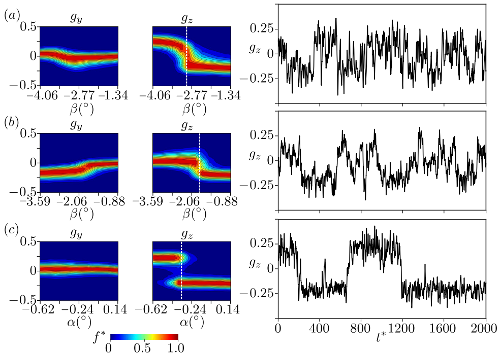
FIGURE 12. Evolution of the base pressure gradients characteristics along the three paths as displayed in figure 10(b): (a) p_{I-IIA} : \alpha = 1.32^\circ , C^* = 0.1 , (b) p_{I-III} : \alpha = 0.42^\circ , C^* = 0.1 , (c) p_{I-V} : \beta = 0^\circ ; C^* = 0.1 . Left: normalised probability density function of the gradient components along the path. Right: time series of vertical pressure gradient g_z for the configuration marked by white dash line in the left figure.
