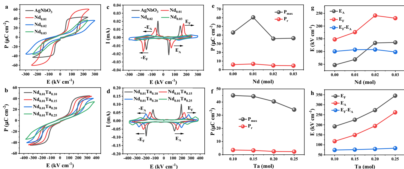
Fig. 3. Compositional variation of antiferroelectric properties under maximum electrical fields: a, b, P-E loops; c, d, I-E curves; e, f, Changes of P_{\max} and P_r ; g, h, Changes of E_F , E_A ; and E_F-E_A , as a function of Nd and Ta concentration.
