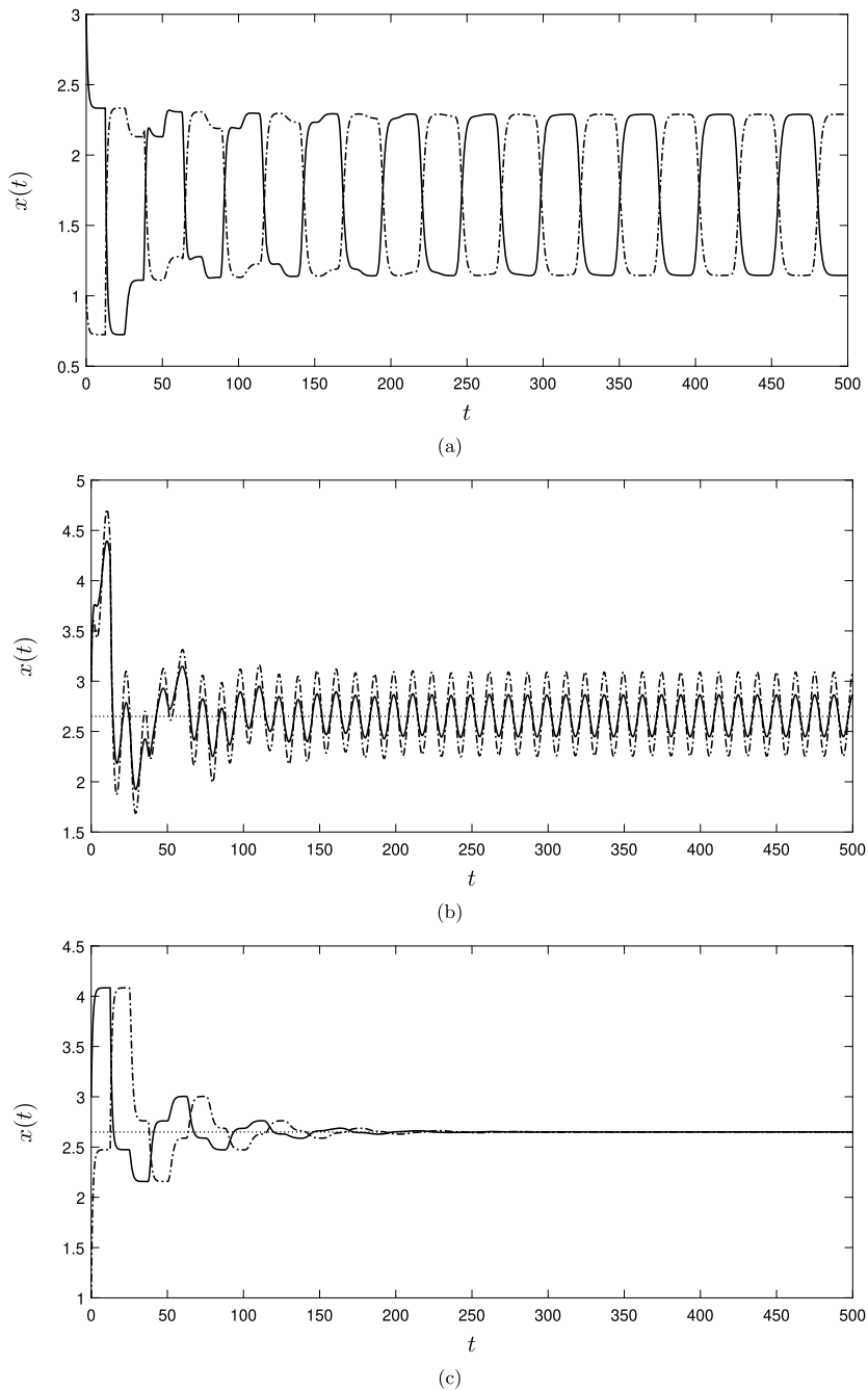
Fig. 4 Numerical solutions of the delay-differential equation (6.1) from Example 6.2, with model data (6.3)–(6.5). The dotted line corresponds to x^\sharp . In panels (a) and (c) the solid and dashed-dotted lines correspond to initial conditions \xi_1 and \xi_2 , respectively. In panel (b), the solid and dashed-dotted lines correspond to forcing terms v_1 and v_2 , respectively. Only initial condition \xi_1 is used. (a) Persistent fluctuations are observed with v = 0 . (b) Bounded oscillations around x^\sharp are observed with v_1 and v_2 as in (6.6). (c) Convergence is observed with constant v = \psi
