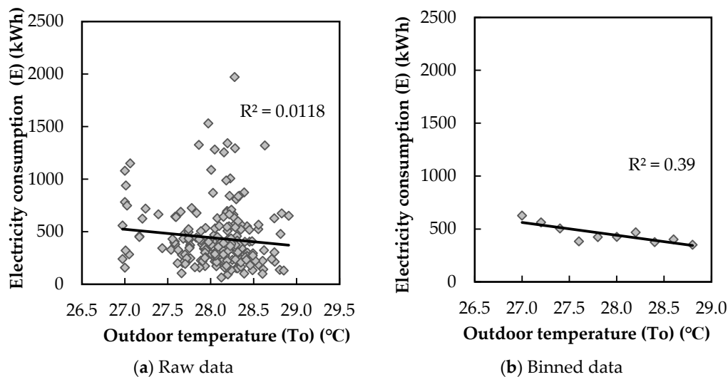
Figure 9. Correlation between outdoor temperature vs. electricity consumption.
