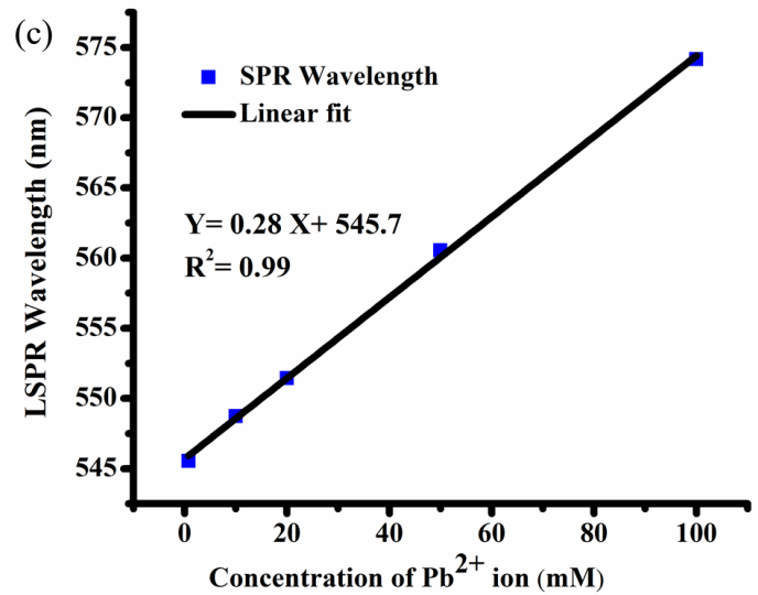
Fig.9. Response of MUA-coated fiber in (a) the Lead Nitrate (LN) solution (b) After removed from LN solution, dried and monitored in air (c) Pb^{2+} concentration versus LSPR wavelength
