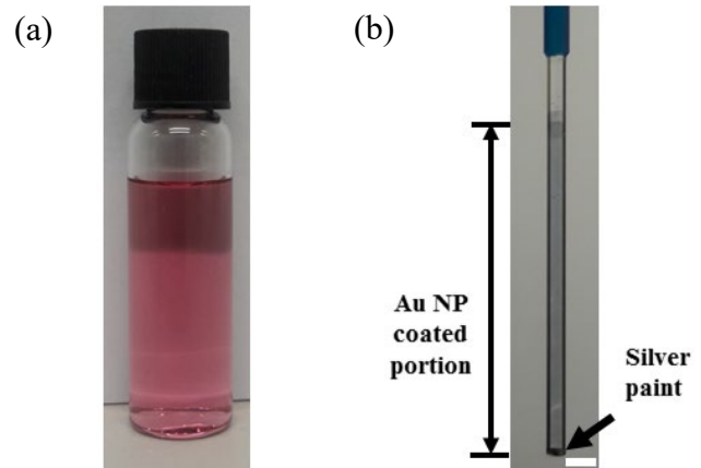
Fig.1 (a) Colloidal Solution (b) Image of the Au NP coated fiber, where the coating area is clearly visible. The white bar at the bottom right represents the reference scale (1 mm).
