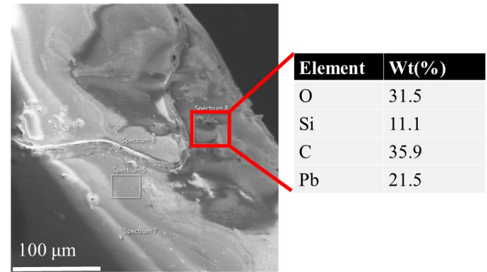
Fig.8. SEM image of Au-MUA-coated fiber after immobilization in Lead Nitrate (LN) solution. The table shows the EDAX analysis of the highlighted section.
