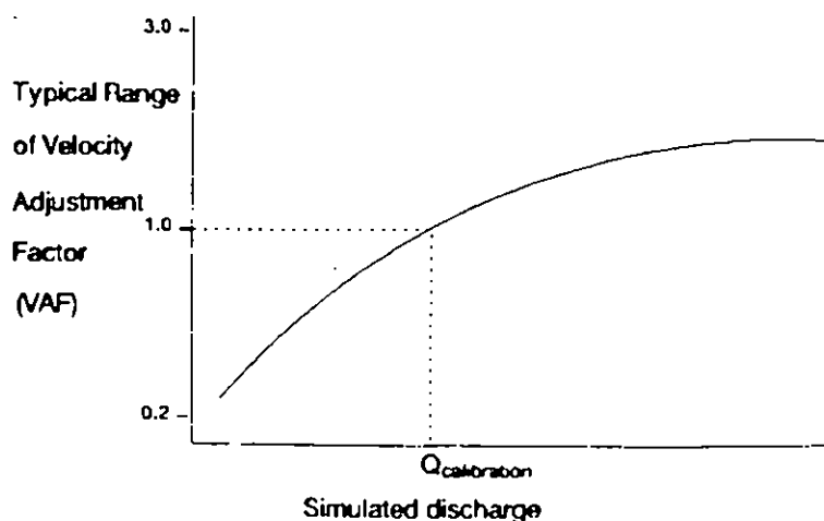
Figure 2.6 Relationship of the Velocity Adjustment Factor with discharge necessary to model variable Mannings n .
