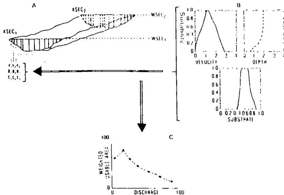
A schematic representation of the IFIM process. Velocity (A), depth (D), and cover/substrate (C) values from various cross sections (XSEC) are combined with water surface elevations (WSEL) at a steady discharge to drive the hydraulic model (steady or dynamic flow) which provides stage/discharge information to PHABSIM [A]. The habitat suitability information [B] is linked to the simulation of cell-by-cell hydraulics to predict (via HABSTAT) the amount of weighted usable area at any proposed discharge [C].
