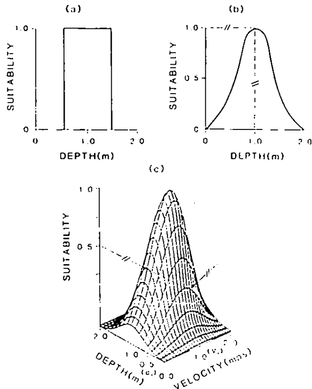
Figure 28 Examples of the three formats of habitat criteria: (a) binary, (b) univariate curve, (c) multivariate response surface
