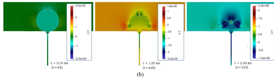
Figure 10. Pressure (a) and vertical velocity component (b) distribution in a central vertical plane for a non-cleaving water drop impacting a 100 \mu\text{m} gap at 0.5 \text{ m/s} . Dimensionless time, scaled by the impact velocity and gap width ( \tau = U_0 t/w ) is indicated in parentheses.
