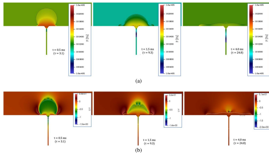
Figure 11. Pressure (a) and vertical velocity component (b) distribution in a central vertical plane for a cleaving ethanol drop impacting a 100 \mu\text{m} gap at 0.62 \text{ m/s} . Dimensionless time, scaled by the impact velocity and gap width ( \tau = U_0 t/w ) is indicated in parentheses.
