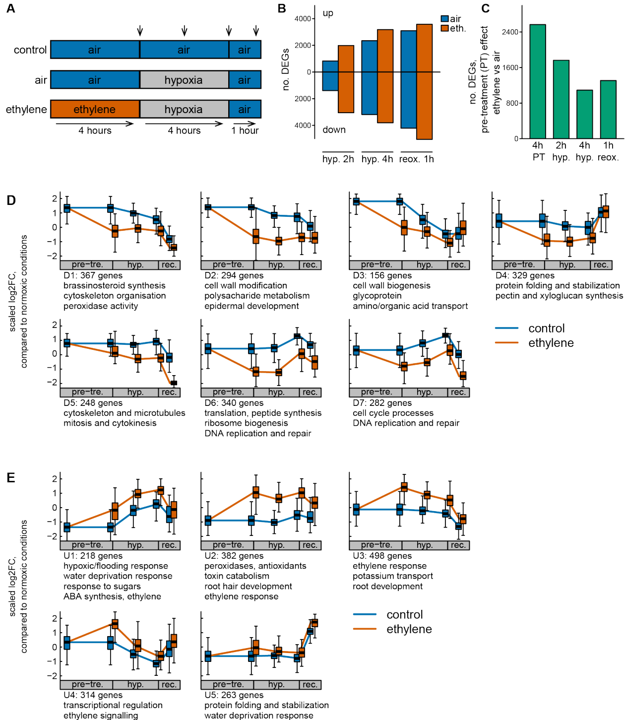
Figure 2. Ethylene leads to transcriptional reprogramming which is maintained during hypoxia and re-oxygenation
