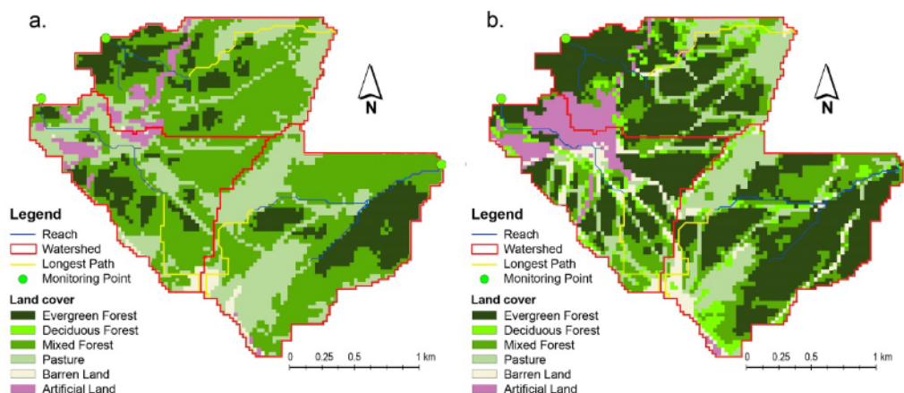
Figure 3. Land cover of the research area for: 1984 (a) and 2018 (b).
