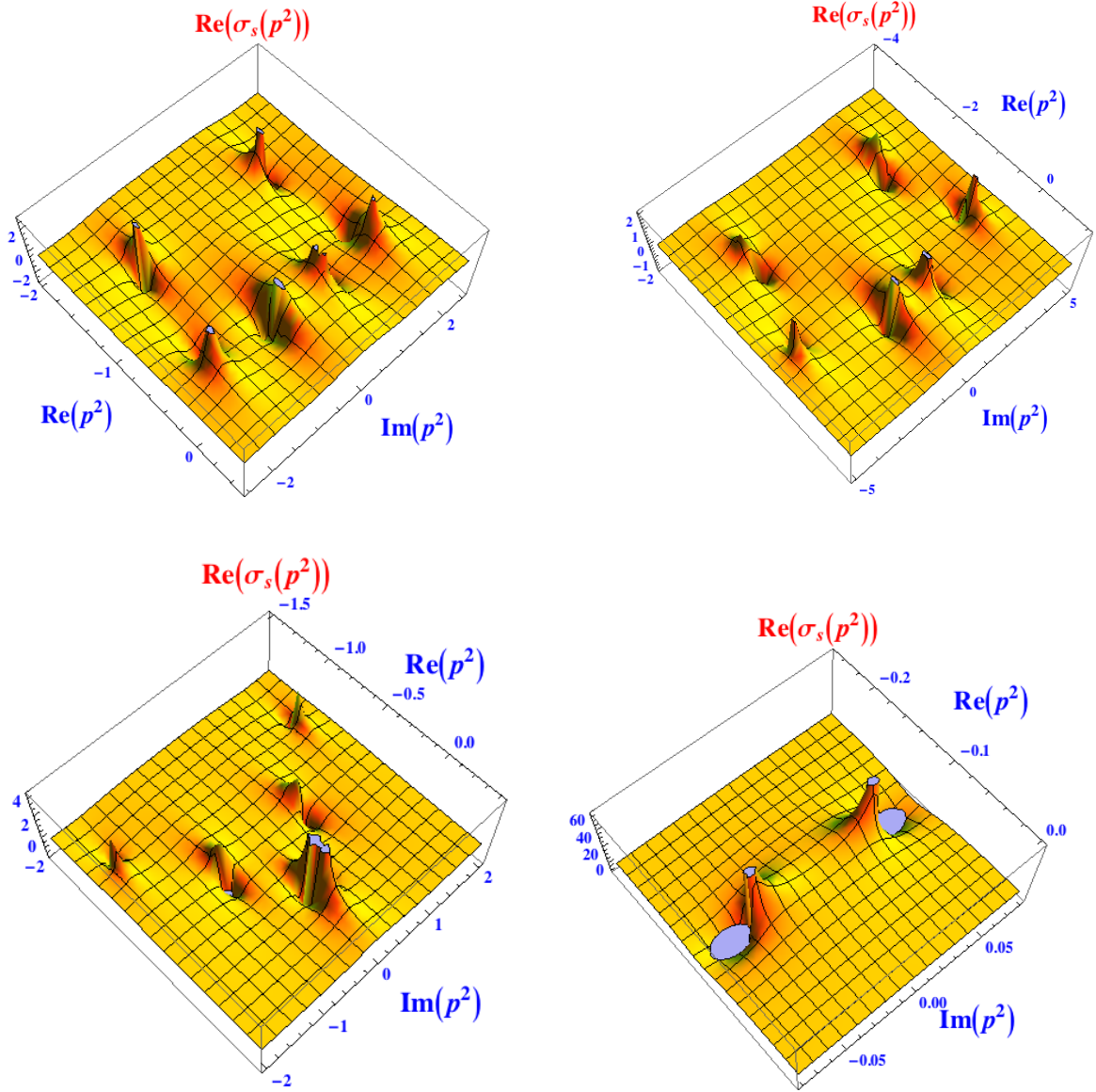
Fig. 1 Scalar function \sigma_s of the light quark propagator S(p) = -i\not{p}\sigma_V(p^2) + \sigma_S(p^2) for the three cases: model 1 in Ref. [23] with \omega D = (0.8 \text{ GeV})^3 , \omega = 0.4 \text{ GeV} , in rainbow-ladder truncation (top-left graph); model 2 in Ref. [23] with \omega D = (1.1 \text{ GeV})^3 , \omega = 0.6 \text{ GeV} , in rainbow-ladder truncation (top-right graph); Ball-Chiu vertex with \omega D = (0.55 \text{ GeV})^3 , \omega = 0.5 \text{ GeV} (bottom-left and -right graph). In all cases the interaction of Ref. [50] is used with a renormalized running quark mass m(19 \text{ GeV}) = 3.4 \text{ MeV} .
