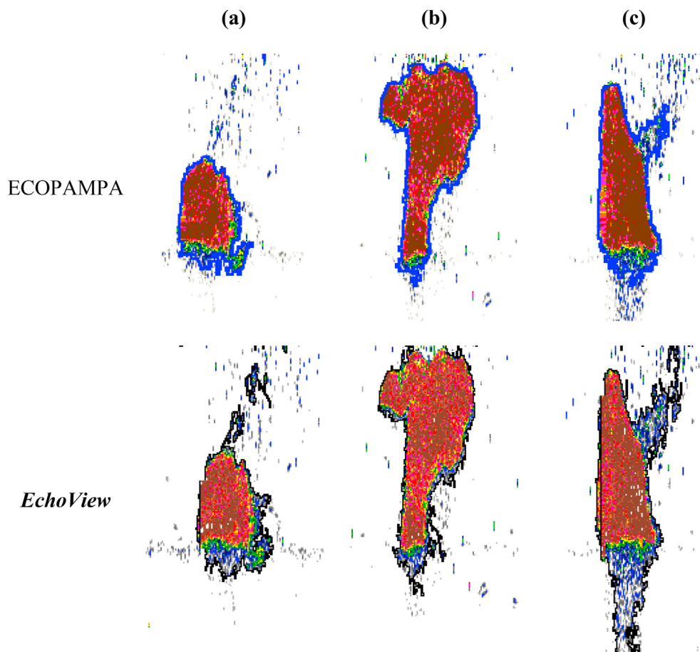
Figure 5. Comparison of detection algorithms between EchoView™ and ECOPAMPA software.
