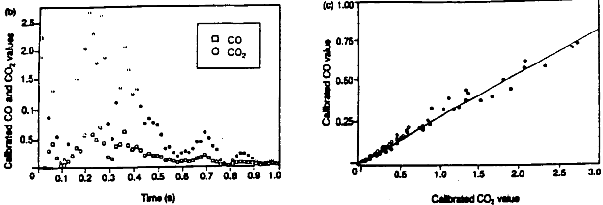
Figure 2 (b) raw data converted to calibrated CO and CO 2 values vs. time using a 10.16 cm calibration cell, and (c) the final CO/CO 2 correlation graph used to obtain unitless slope.
