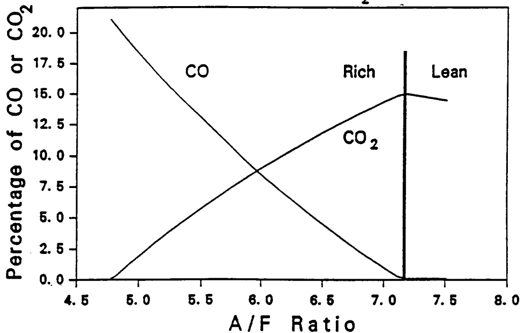
Figure 5 A gasoline engine combustion graph showing calculated CO and CO_2 emissions as a function of molar air-to-fuel ratio. The solid vertical line represents stoichiometry.
