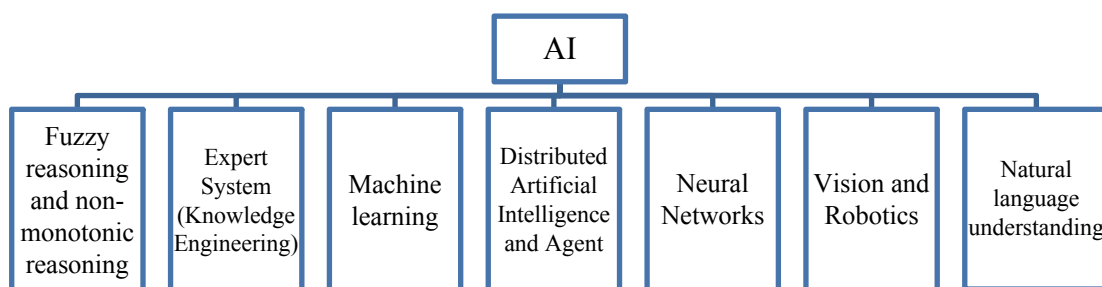
Figure 9-Classification of AI
