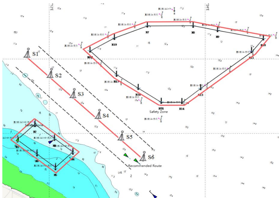
Figure 4.4 The Safety Zone and Recommended Route of Binhai OWF Source: Produced by the author.
