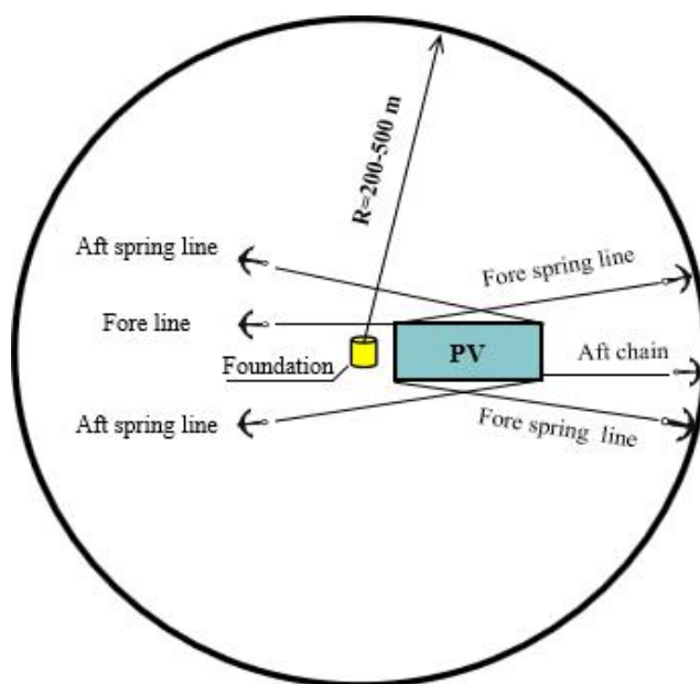
Figure 2.2 Anchoring drawing of the PV
