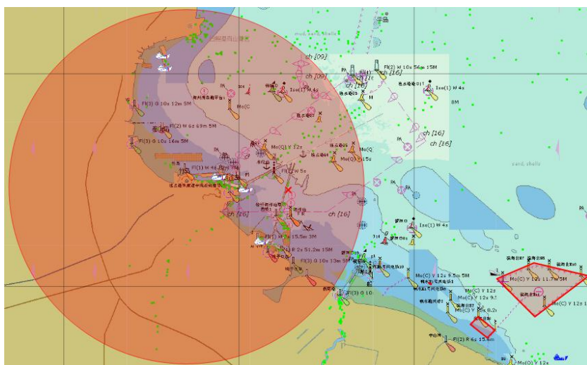
Figure 4.5 Signal coverage of Lian Yungang coast station Source: Produced by the author.
