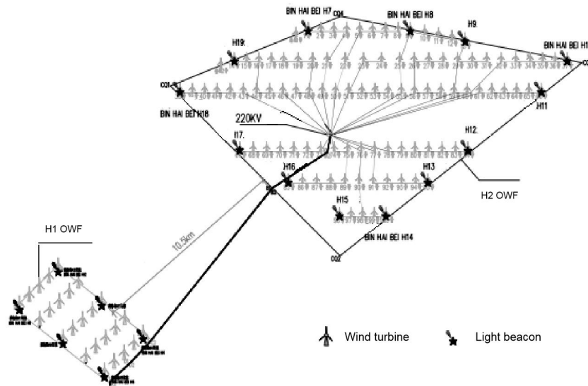
Figure 4.3 Site plan of Binhai OWF
