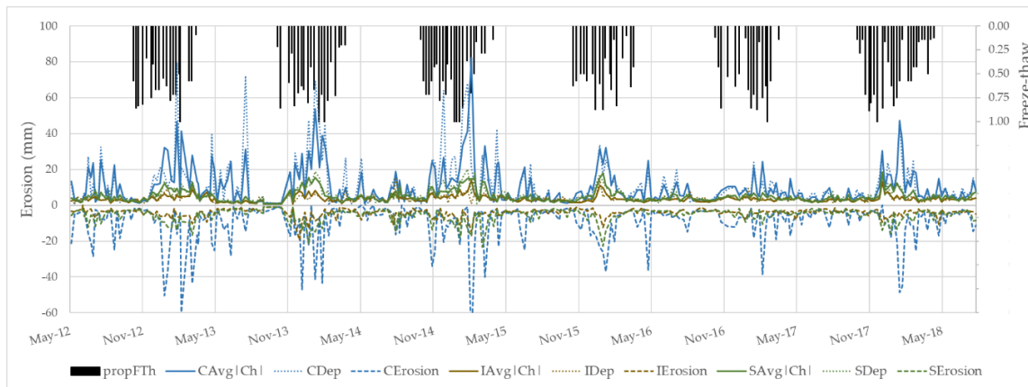
Figure 6. Time series of erosion parameters with freeze-thaw variables shows a seasonal pattern and lagged relationship between onset of freeze-thaw events and peak of erosive activity.
