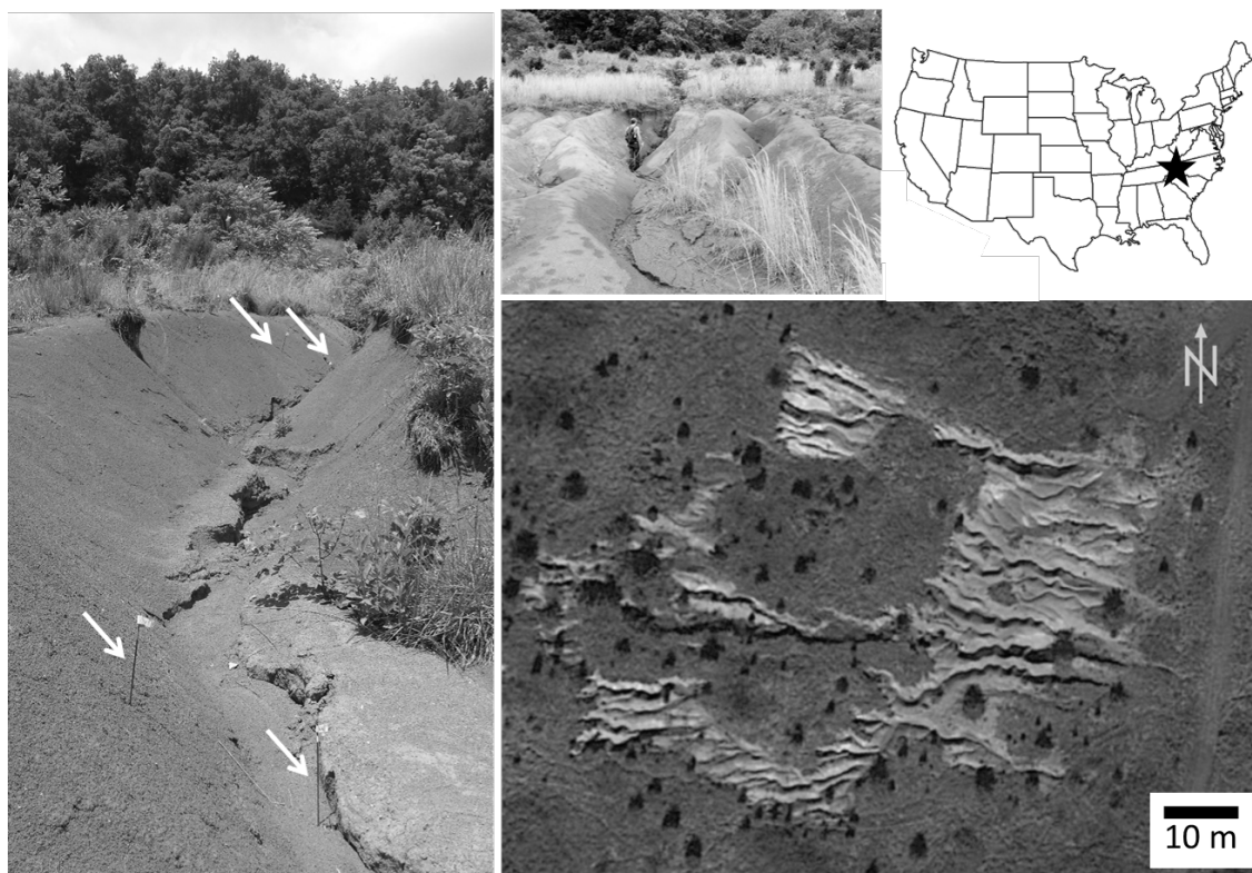
Figure 1. Study site location and representative gully, showing interfluves, sidewalls, and channels. Erosion pins are indicated by arrows.
