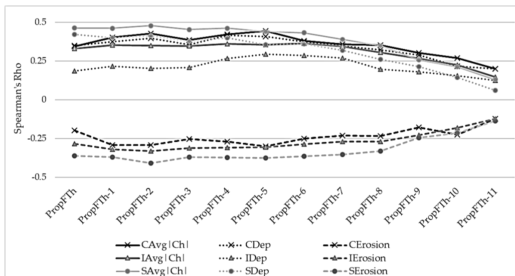
Figure 5. Cross correlation of lagged freeze-thaw variable with erosion parameters.
