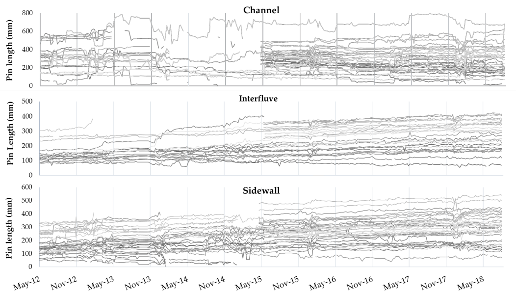
Figure 3. Each series represents a single erosion pin measured at weekly intervals. Length of erosion pins increases over time for channels, interfluves, and sidewalls. New pins were added in 2015 to replace pins eroded out during prior seasons.
