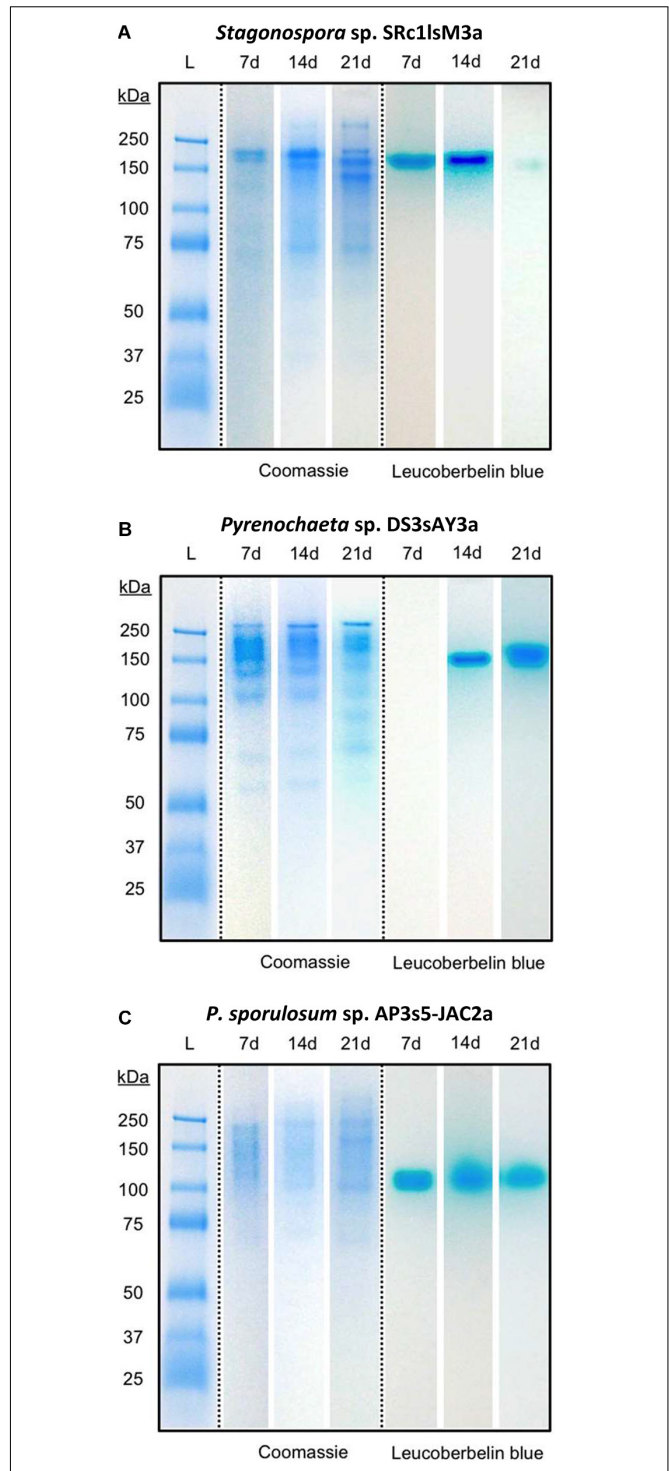
FIGURE 3 | Fungal extracellular enzymes directly oxidized Mn(II). Native PAGE of secretome samples from all 3 time points for (A) Stagonospora sp. , (B) Pyrenochaeta sp. , and (C) P. sporulosum . Lane L: Pre-stained blue protein molecular mass markers with sizes in kDa to left of images. Center panels: Gel stained with Coomassie G-250 for 1 h. Right panels: Replicate gel of the same secretome samples after incubation with 400 µM Mn(II) for 2 h followed by staining with Leucoberbelin blue, which turns blue in the presence of Mn(III/IV) oxides. Images show 1 biological replicate that is representative of 4 total replicates of each species and time point.
