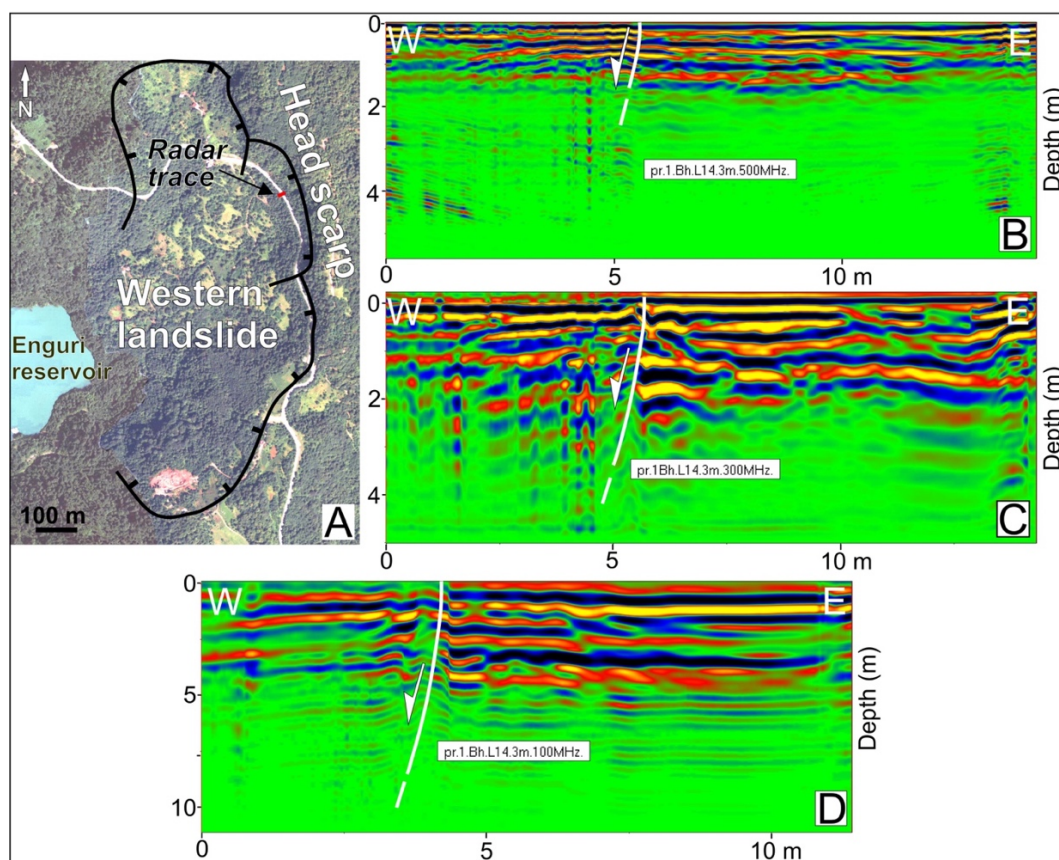
85 86 Figure 11: A. Location of the Ground Penetrating Radar (GPR) survey carried out in the western landslide across one 87 of the active upper slip plane affecting the main road. The black line shows the uppermost head scarp of the landslide. 88 B. GPR sections surveyed with an antenna at: B. 500 MHz, C. 300 MHz, and D. 100 MHz. The white lines represent 89 the same slip plane.
