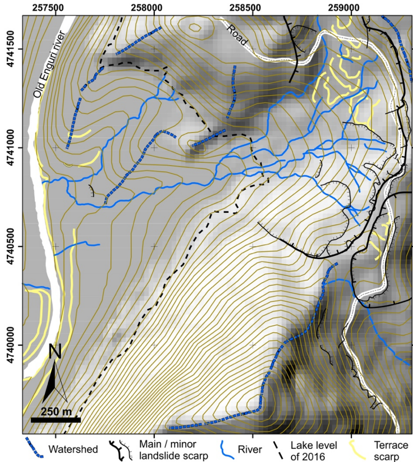
37 Figure 4: Geomorphological map of the area surrounding the western landslide, based on our new field surveys in the 38 onshore zone and data from Zolotarev et al. (1968) for the zone now submerged by the Enguri water reservoir.
