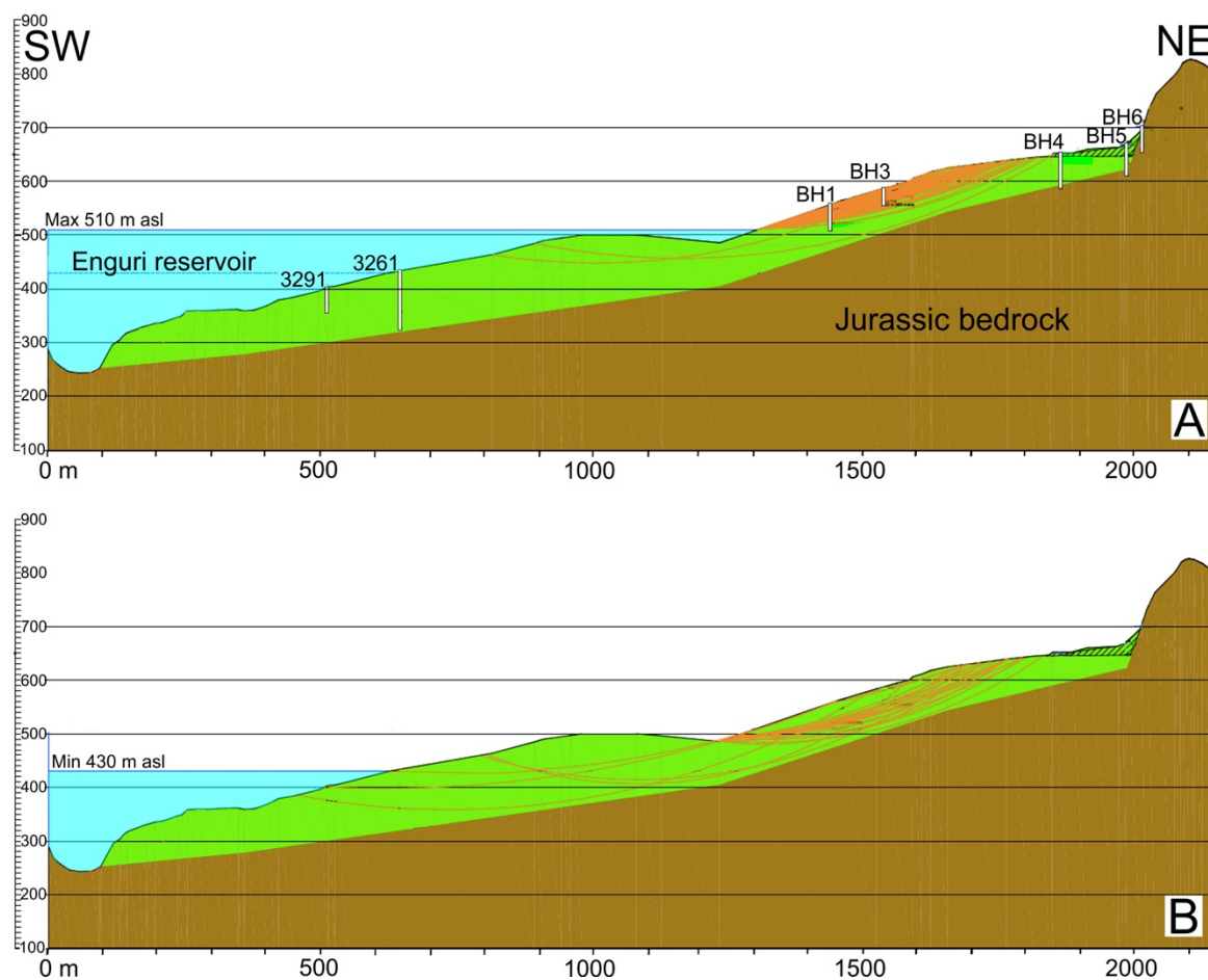
80 Figure 12: Sections of the static numerical modeling developed to analyze the effect of variation of the water level in 81 the main landslide body. A. Instability developed with maximum level of the reservoir water level (orange lines = slip 82 surfaces with FS < 1). B. Analysis of the effect of variation of the reservoir water level down to the minimum level; note 83 new slip surface (with FS < 1) formation at lower elevations.
