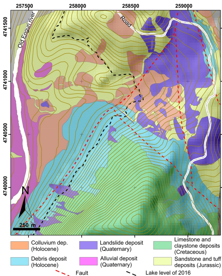
33 Figure 3: Geological map of the area surrounding the western landslide, based on our new field surveys in the onshore 34 zone and data from Zolotarev et al. (1968) for the zone now submerged by the Enguri water reservoir.
