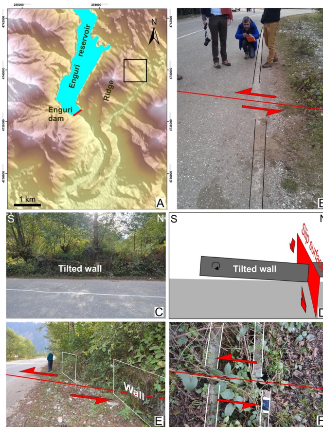
37 38 Figure 8: Features observed at the eastern landslide, located in the box of Figure A. B. Left-lateral offset of the Jvari- 39 Khaishi-Mestia road white strip. C. and D. Photo and interpretation of the tilted wall along the same road. E. Left- 40 lateral offset of 1.9 m of a 1974 AD wall. F. Left-lateral offset of a recent water channel.
