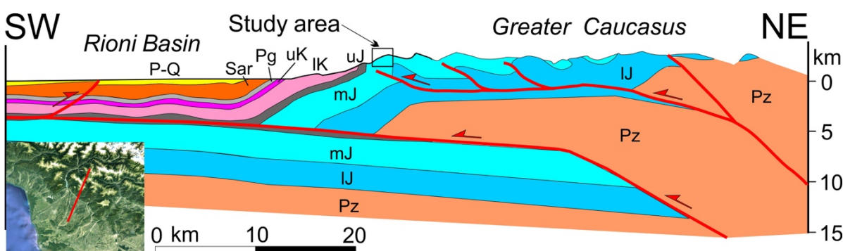
56 Figure 16: Structural section passing through the study area (box), obtained by integrating our field surveys with 57 geophysical and geological data from Banks et al. (1997). Note the presence of a main basal thrust dipping north, which 58 shows a ramp-flat geometry that produced a frontal asymmetric ramp anticline.
