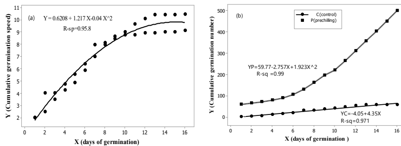
Fig 3. (a) The relationships between cumulative germination speed and time and (b) between cumulative germination number and time.
